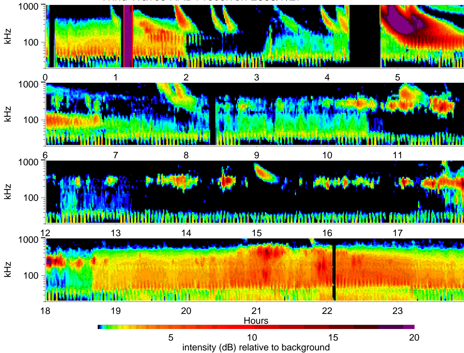
Wind Waves RAD1 receiver: 2005/7/27
