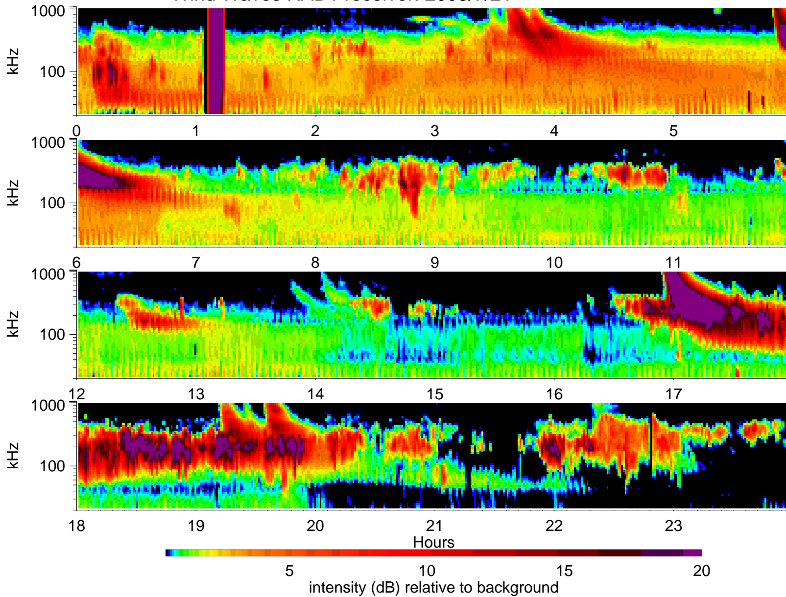
Wind Waves RAD1 receiver: 2005/7/21
