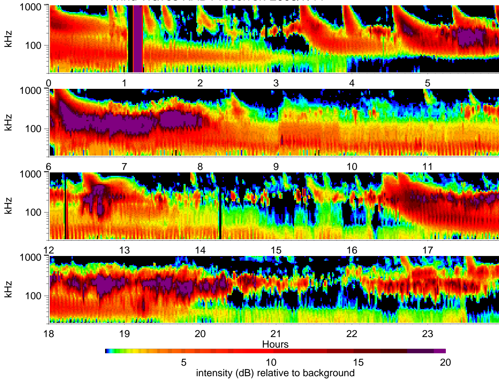
Wind Waves RAD1 receiver: 2005/7/11
