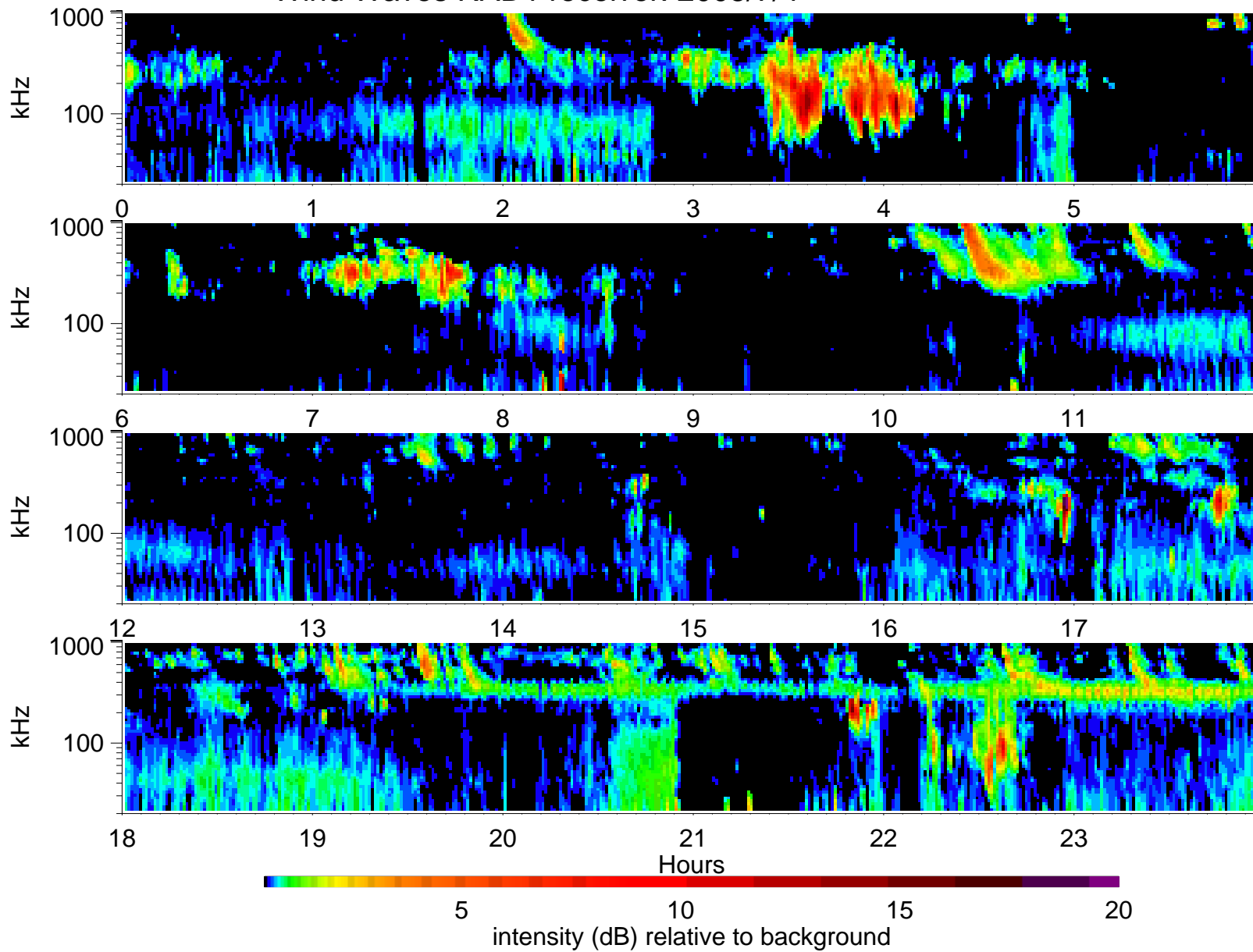
Wind Waves RAD1 receiver: 2005/7/4
