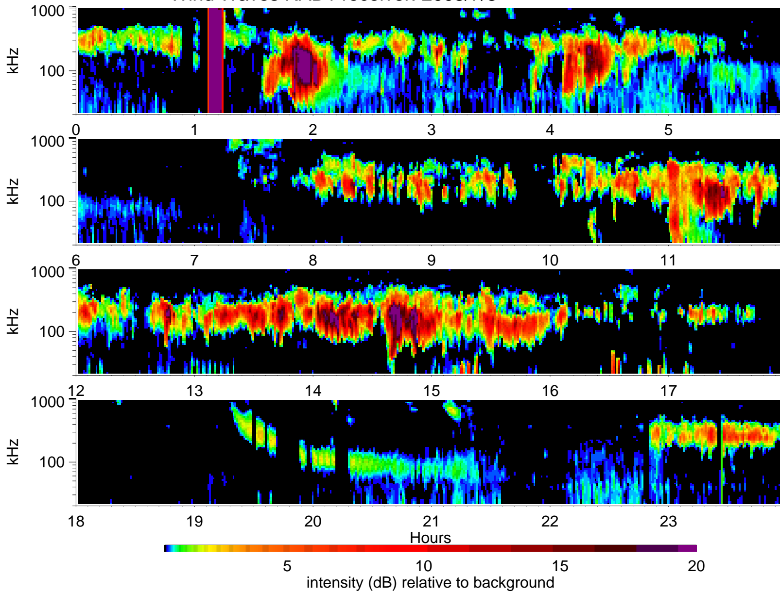
Wind Waves RAD1 receiver: 2005/7/3
