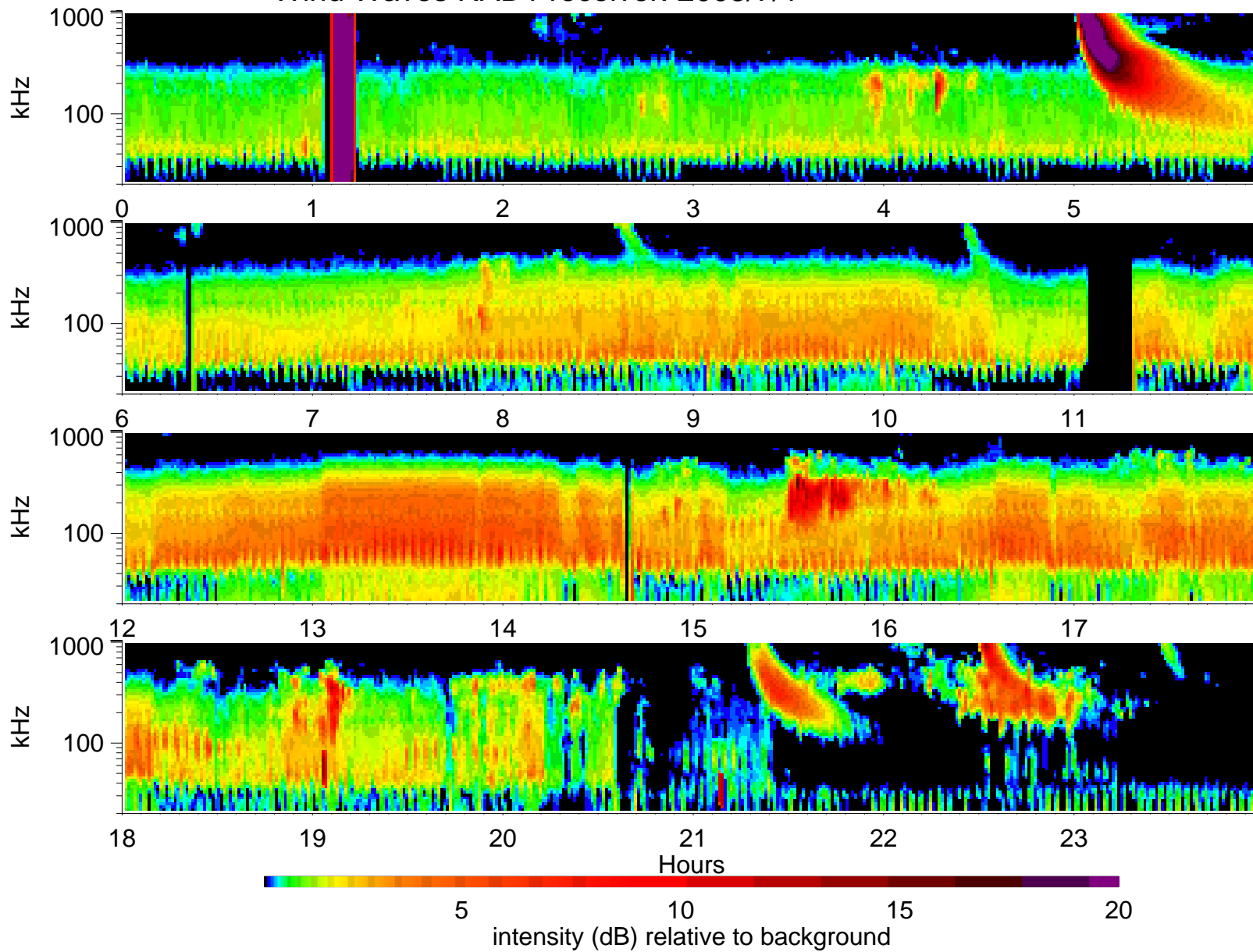
Wind Waves RAD1 receiver: 2005/7/1
