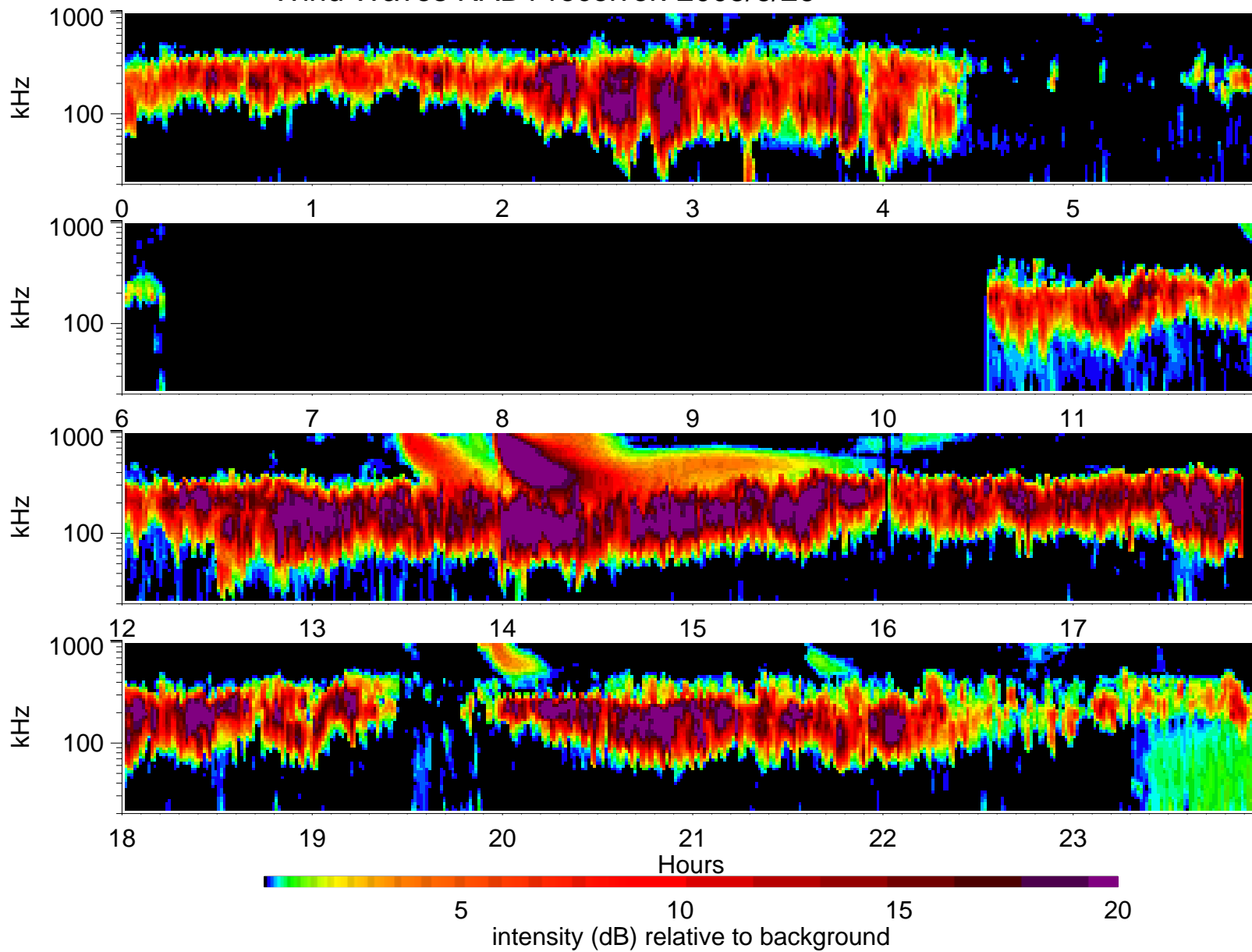
Wind Waves RAD1 receiver: 2005/6/26
