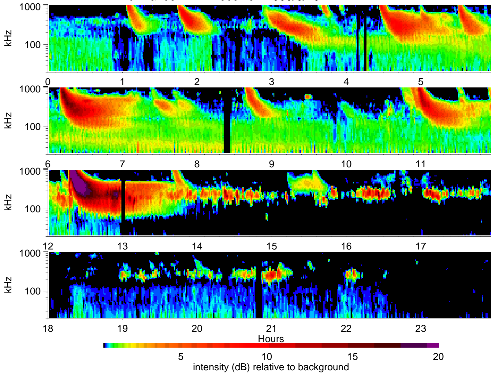
Wind Waves RAD1 receiver: 2005/6/20
