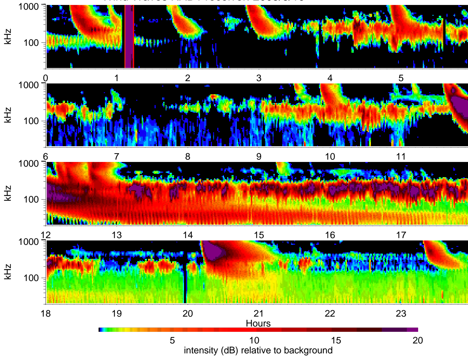
Wind Waves RAD1 receiver: 2005/6/19
