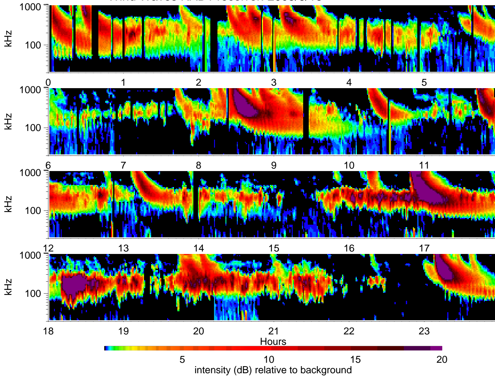
Wind Waves RAD1 receiver: 2005/6/18
