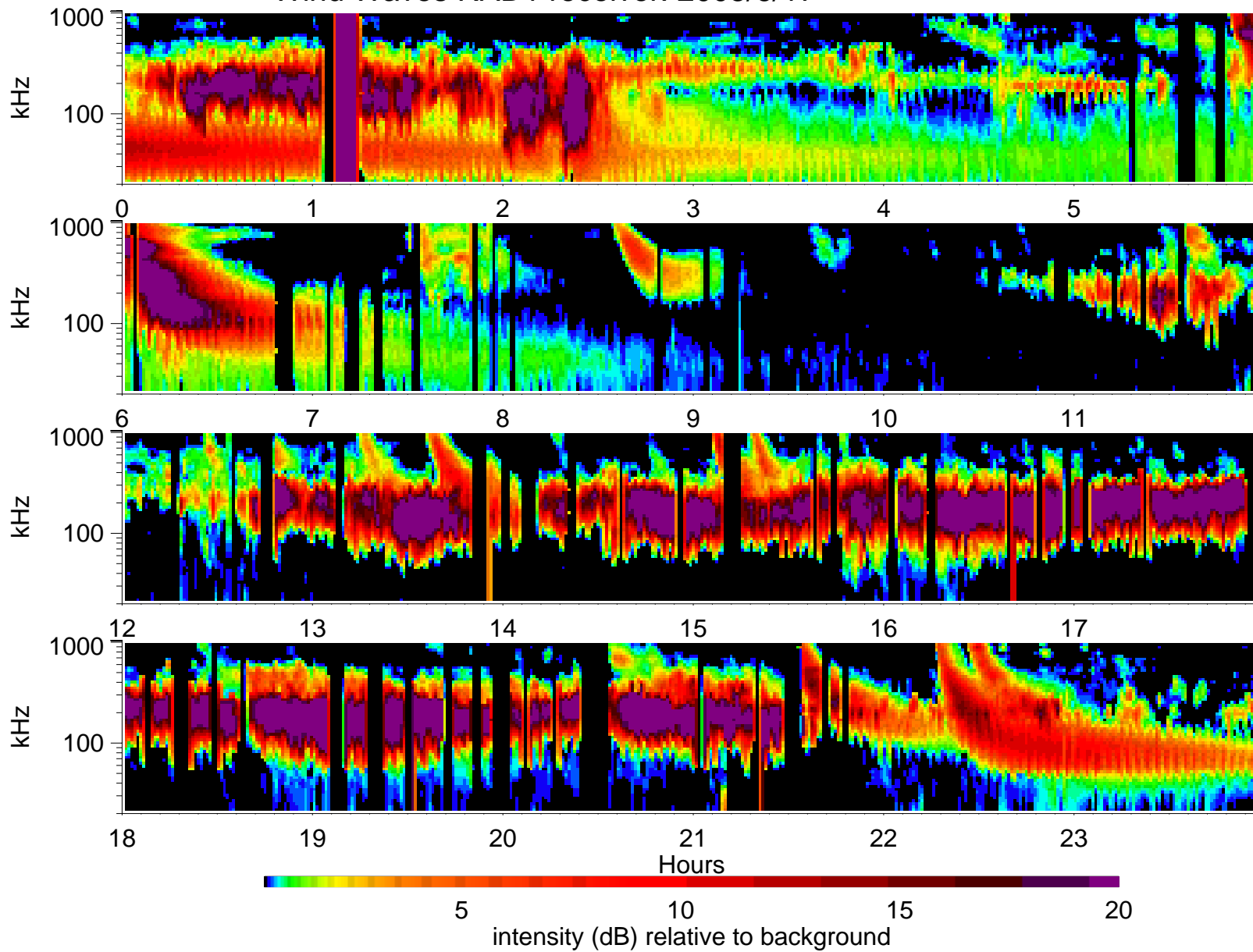
Wind Waves RAD1 receiver: 2005/6/17
