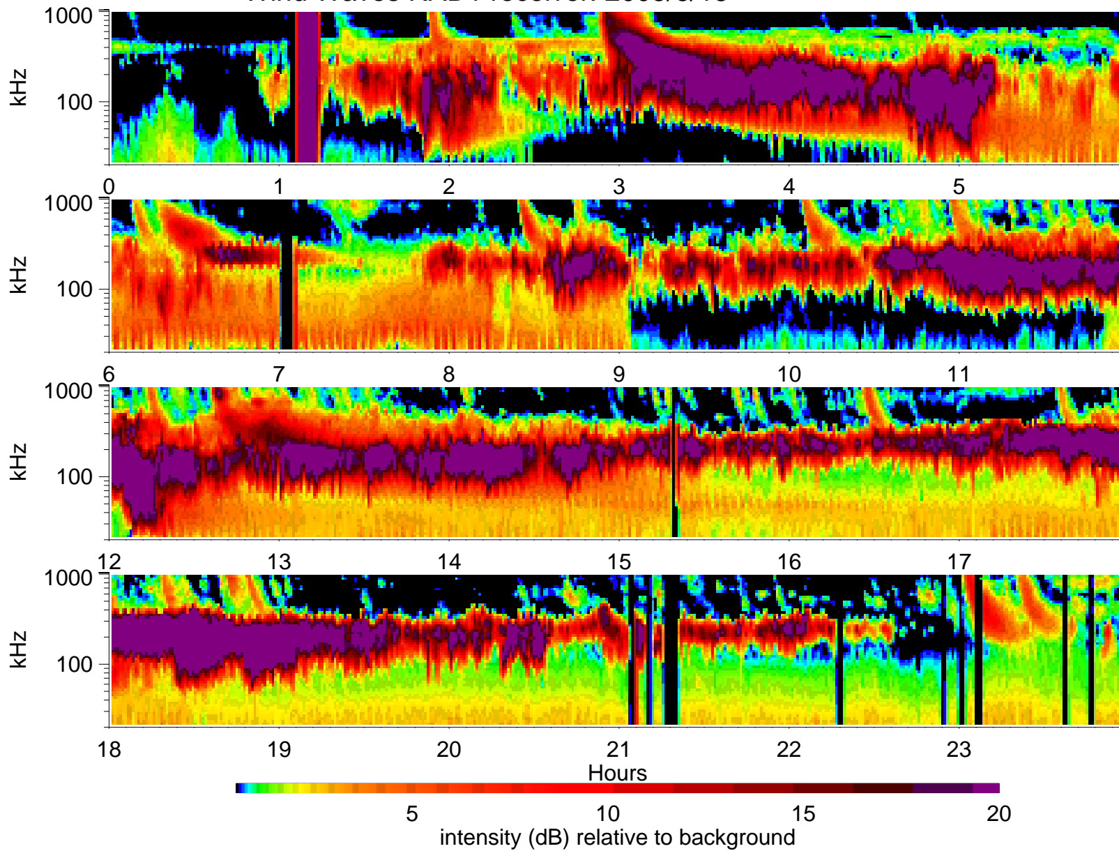
Wind Waves RAD1 receiver: 2005/6/13
