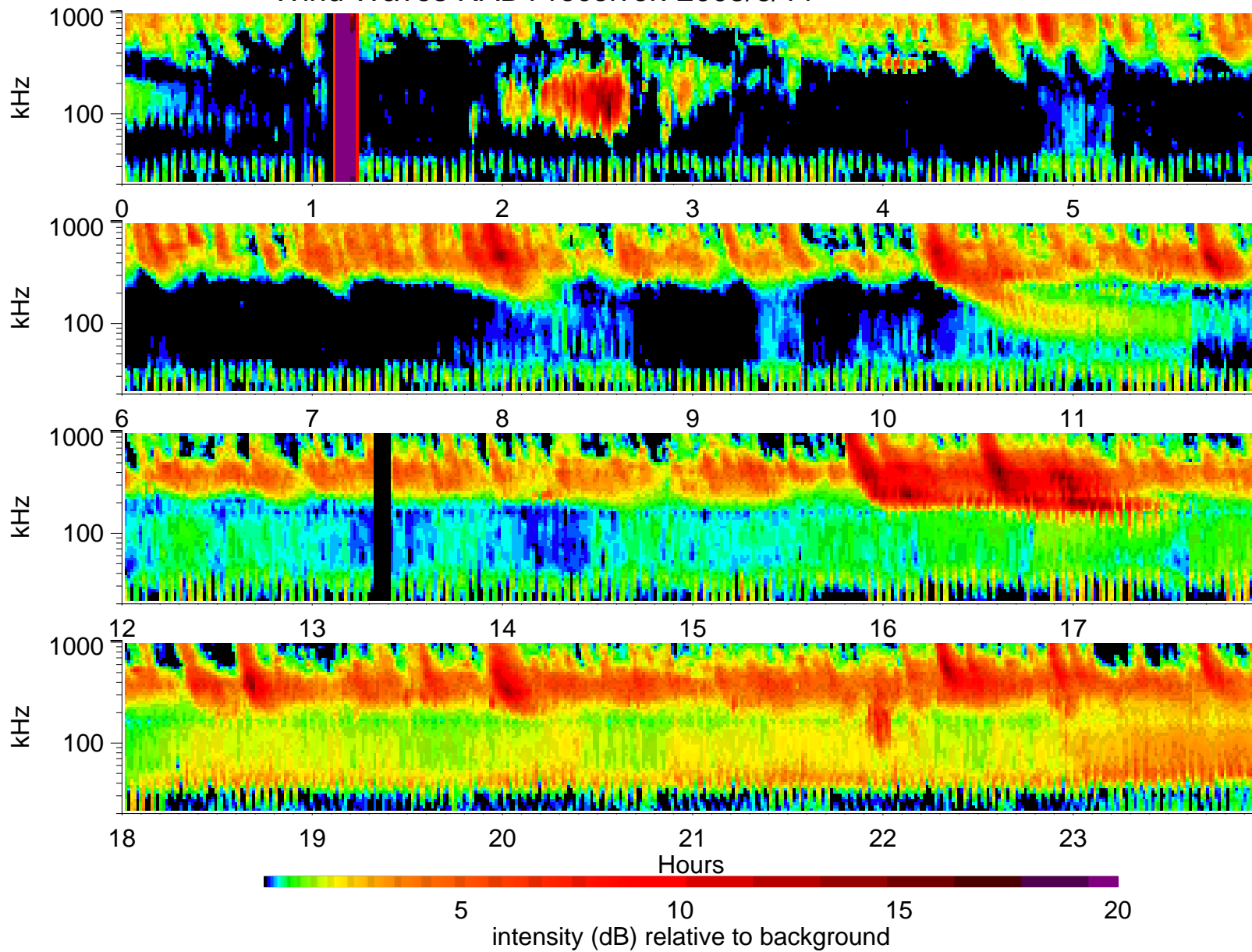
Wind Waves RAD1 receiver: 2005/6/11
