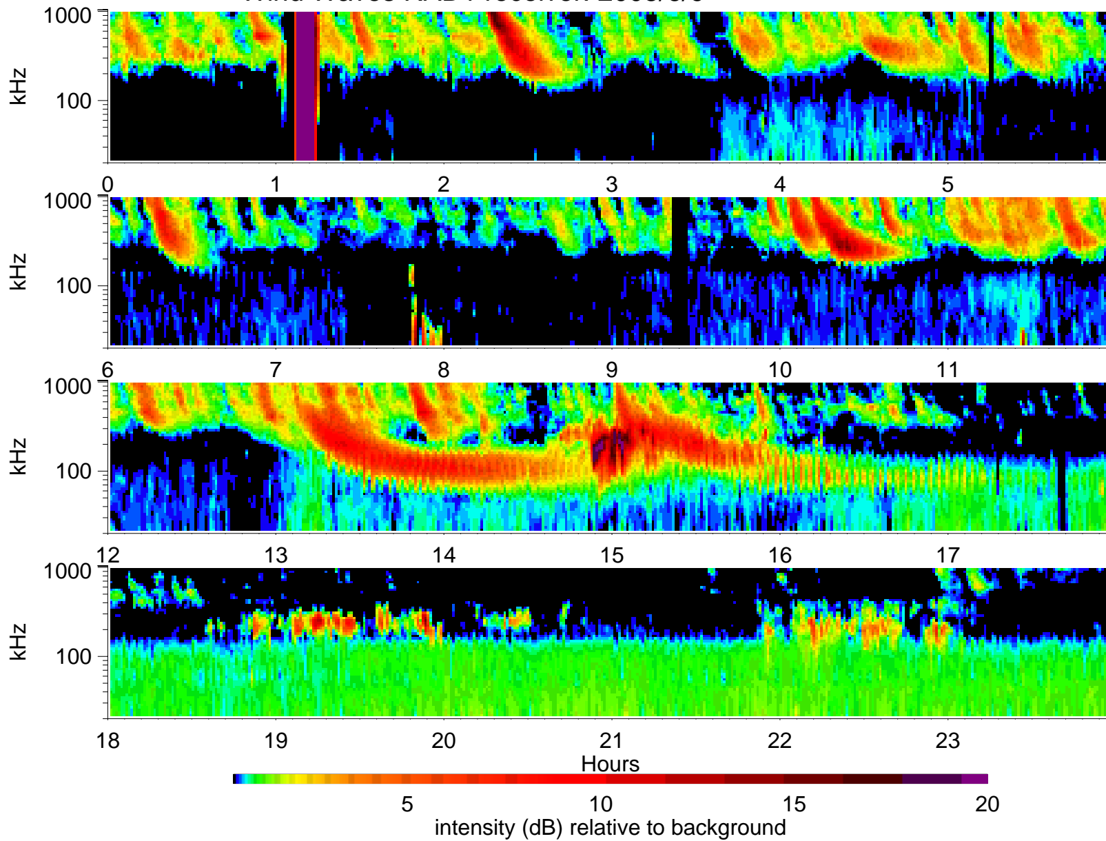
Wind Waves RAD1 receiver: 2005/6/9
