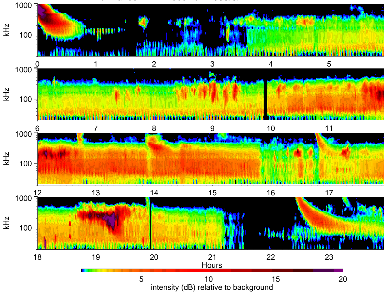
Wind Waves RAD1 receiver: 2005/6/4
