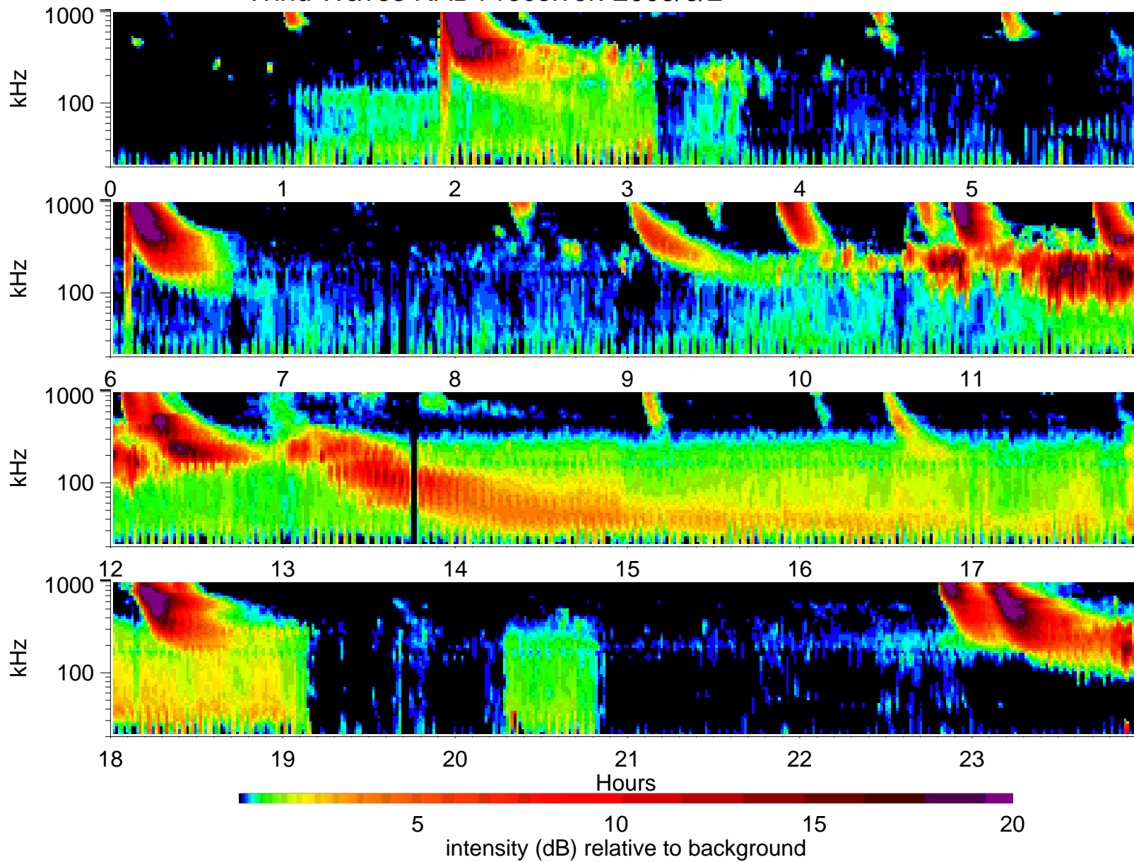
Wind Waves RAD1 receiver: 2005/6/2
