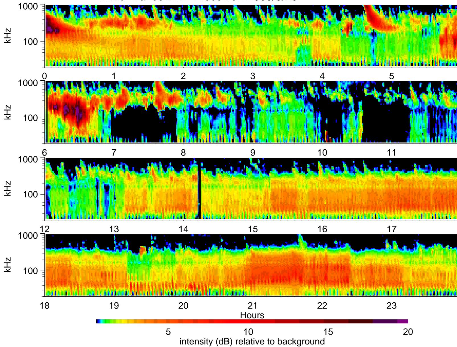
Wind Waves RAD1 receiver: 2005/5/29
