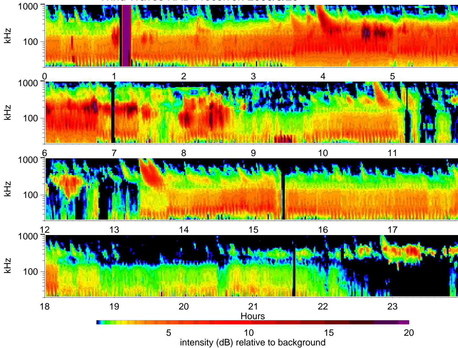
Wind Waves RAD1 receiver: 2005/5/20
