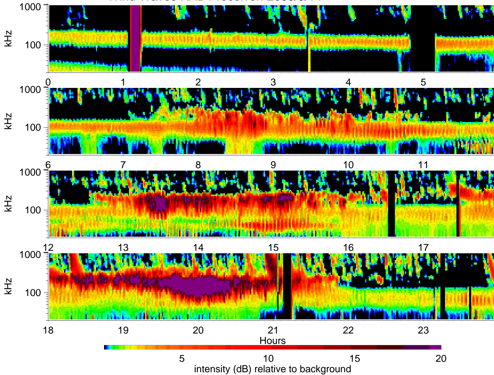
Wind Waves RAD1 receiver: 2005/5/14
