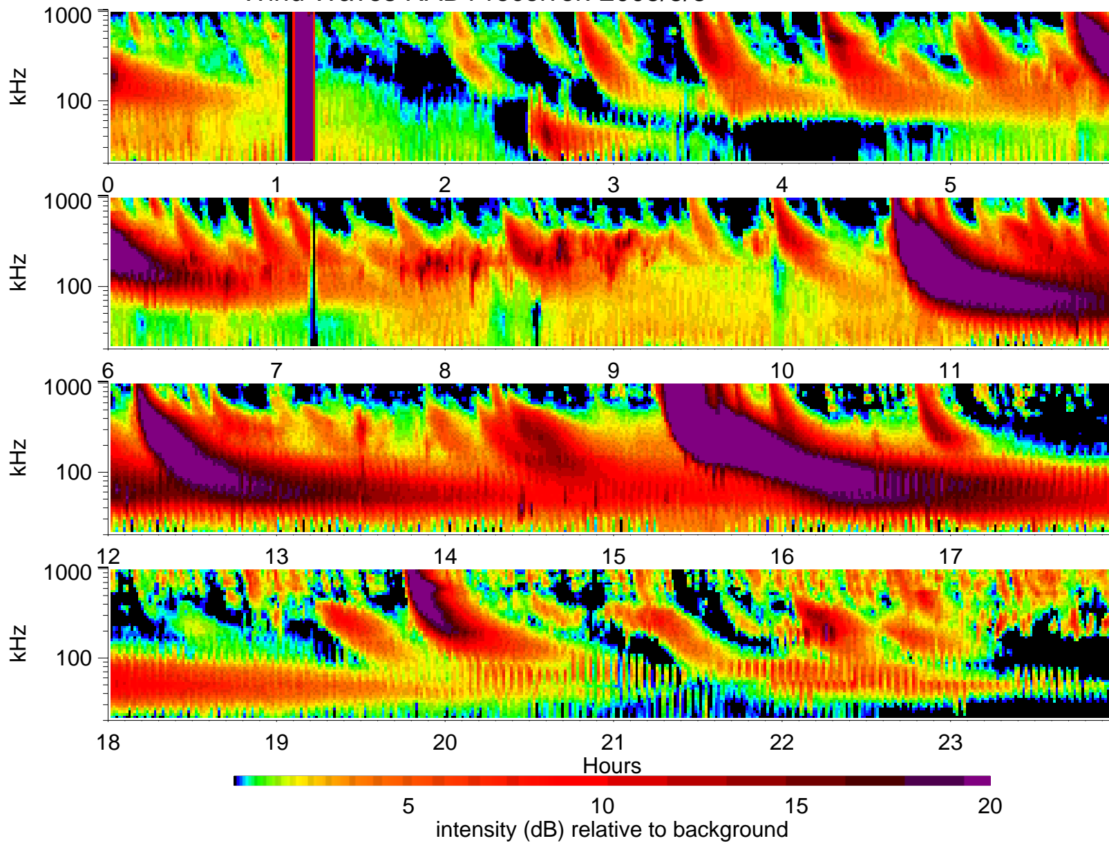
Wind Waves RAD1 receiver: 2005/5/8
