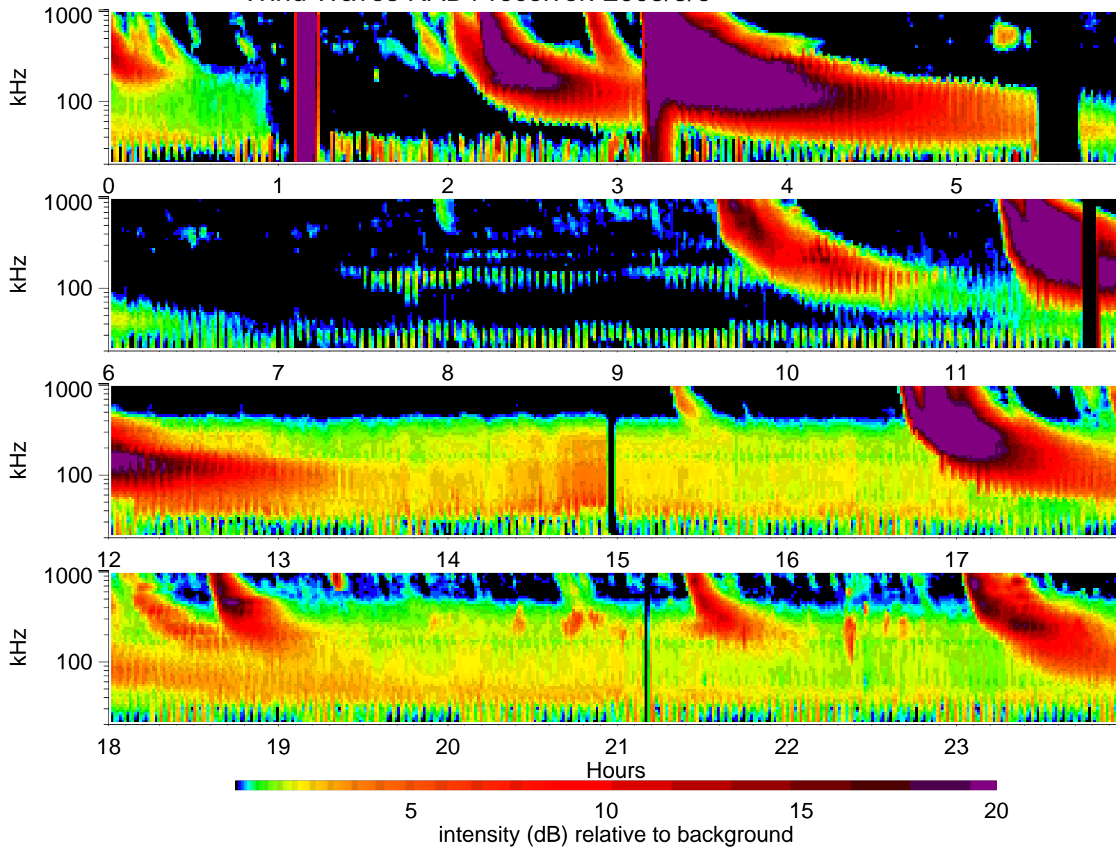
Wind Waves RAD1 receiver: 2005/5/6
