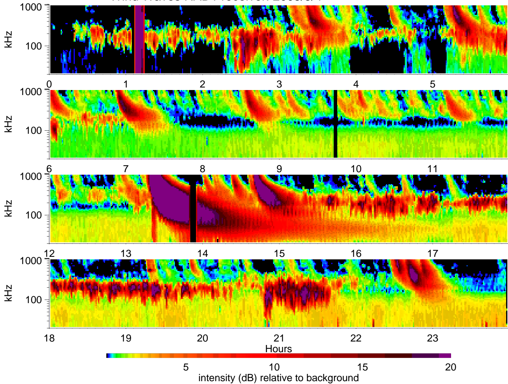
Wind Waves RAD1 receiver: 2005/5/4
