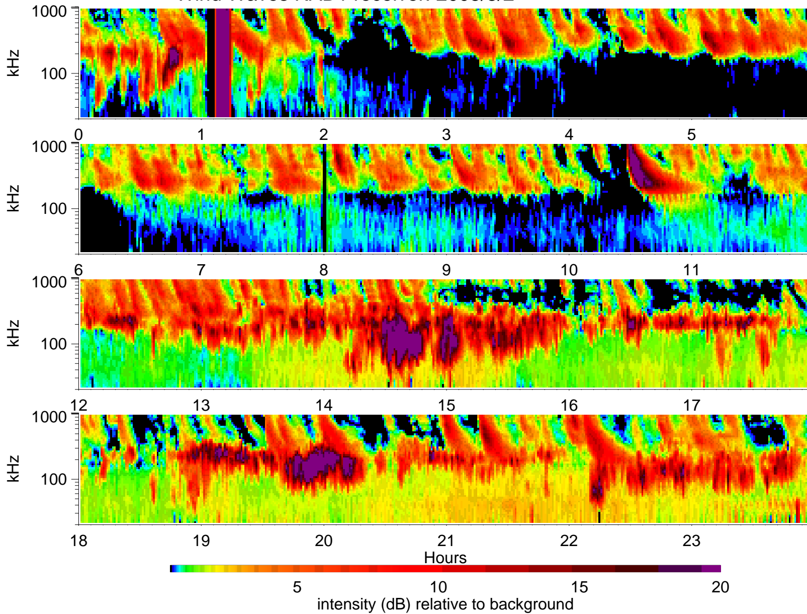
Wind Waves RAD1 receiver: 2005/5/2
