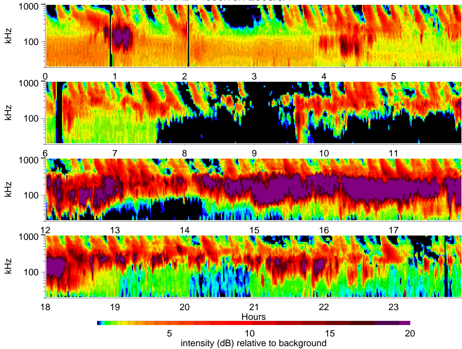
Wind Waves RAD1 receiver: 2005/5/1
