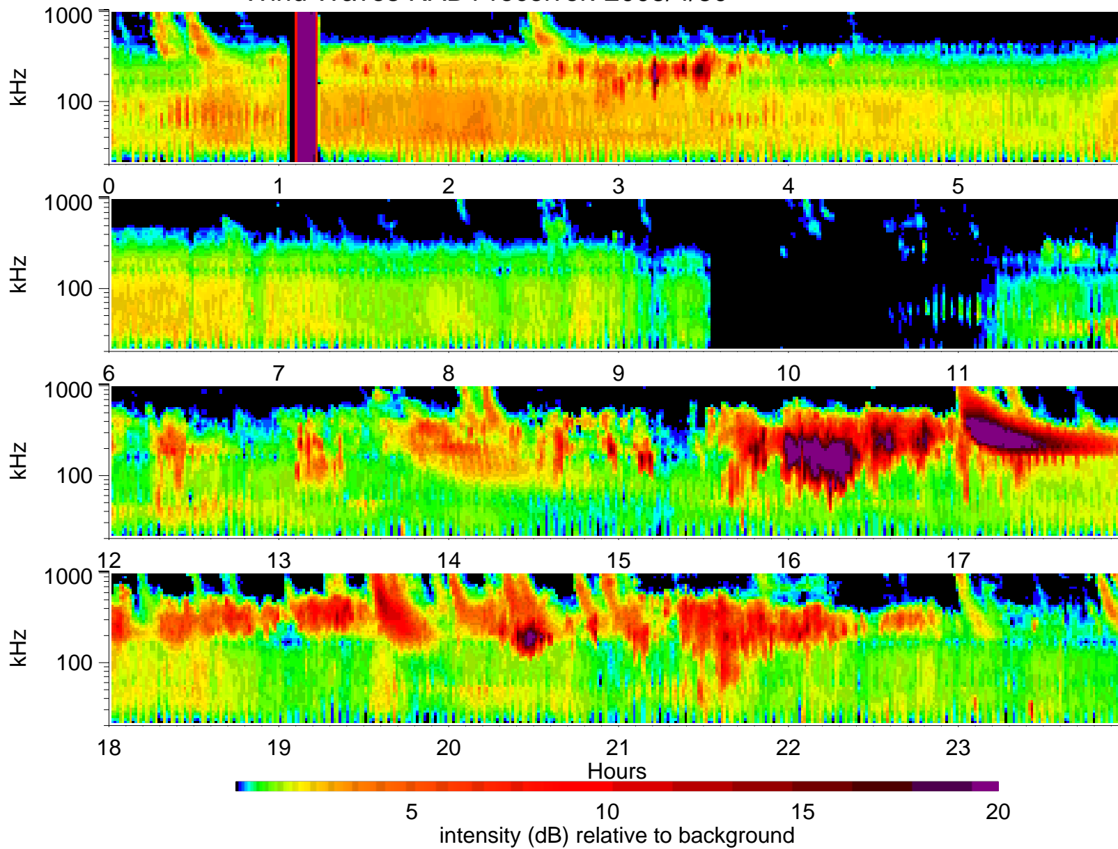
Wind Waves RAD1 receiver: 2005/4/30
