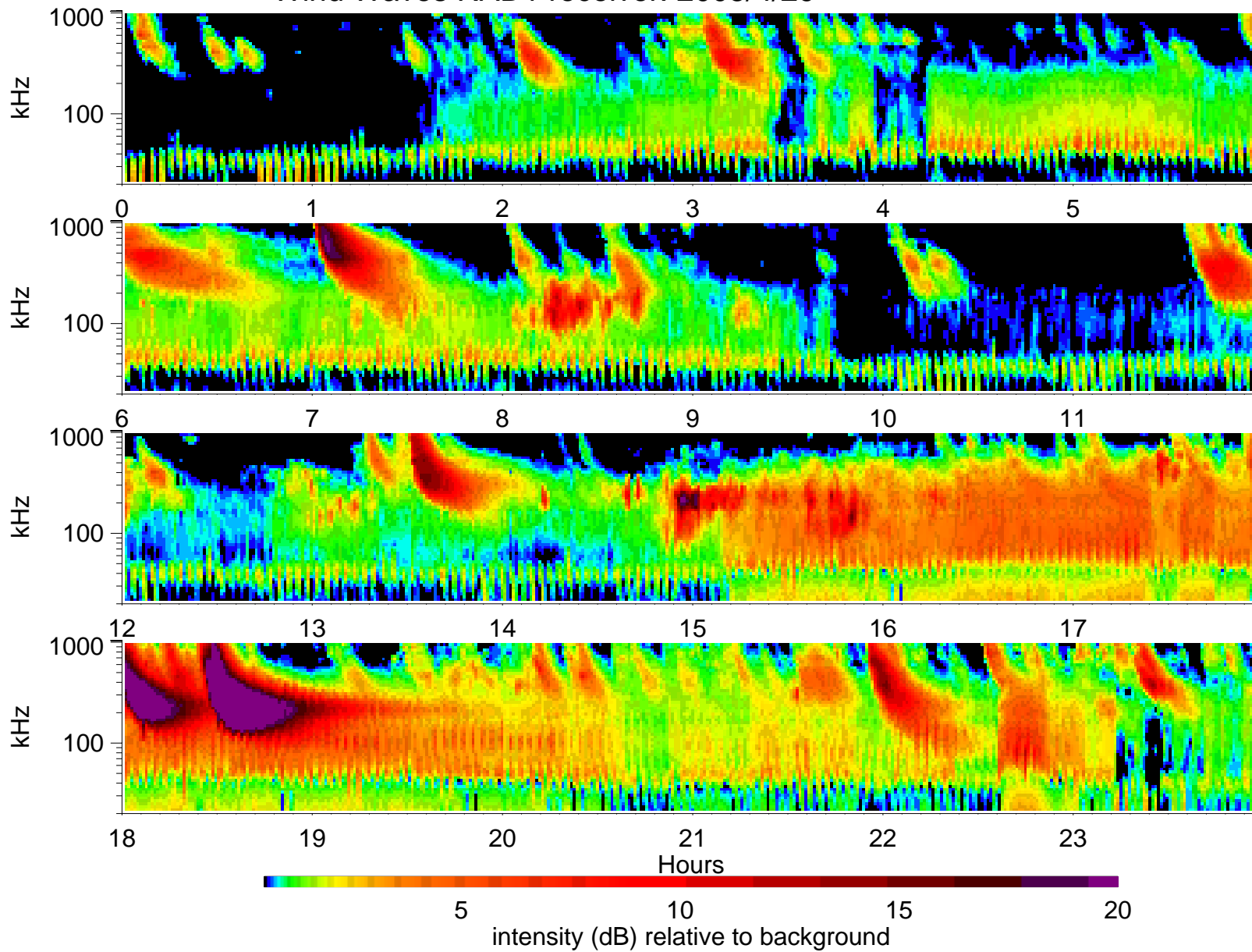
Wind Waves RAD1 receiver: 2005/4/29
