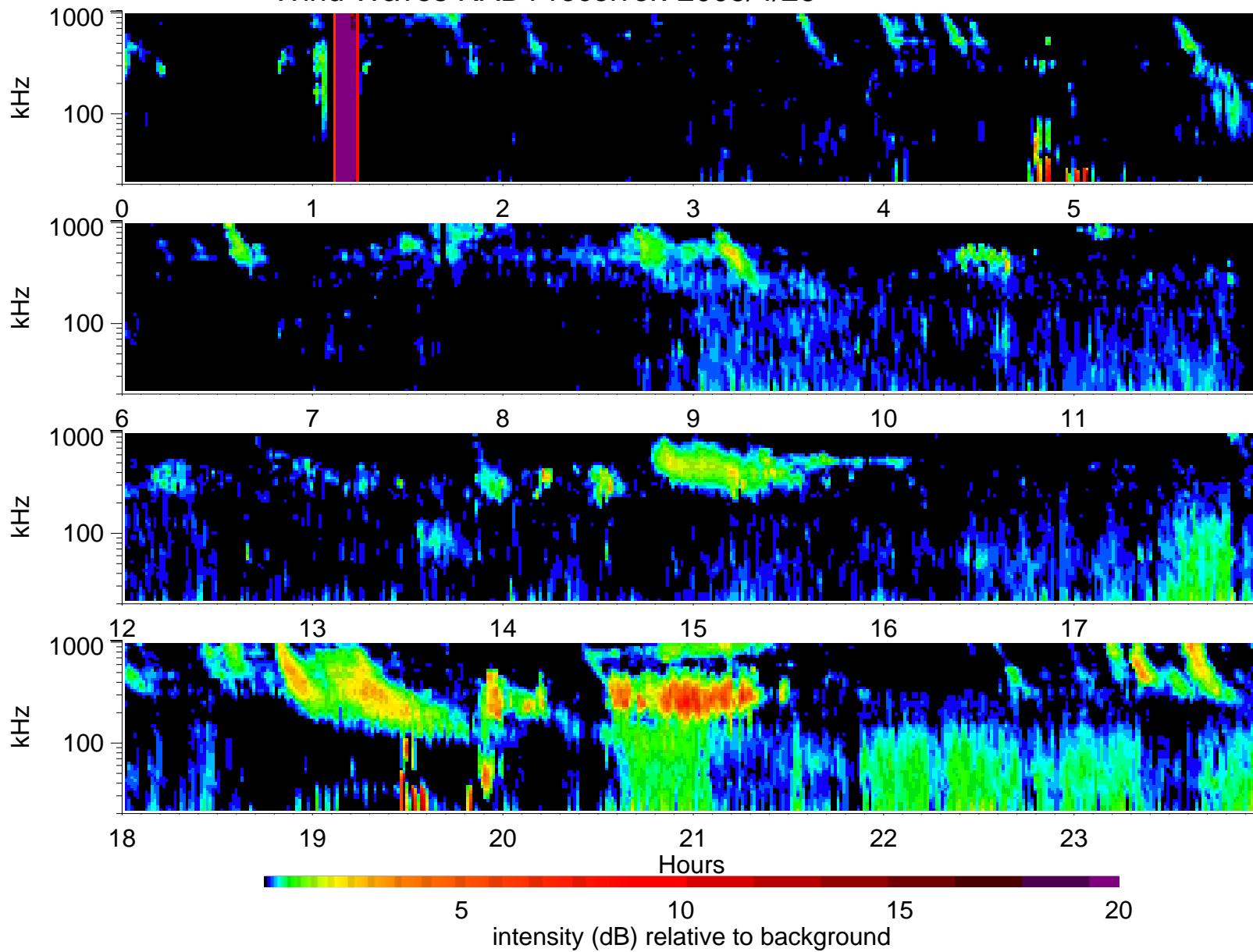
Wind Waves RAD1 receiver: 2005/4/26
