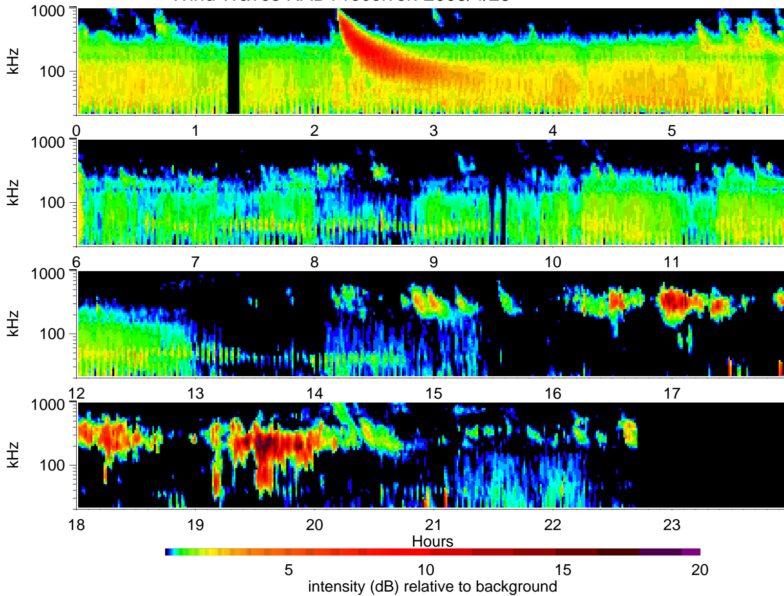
Wind Waves RAD1 receiver: 2005/4/23
