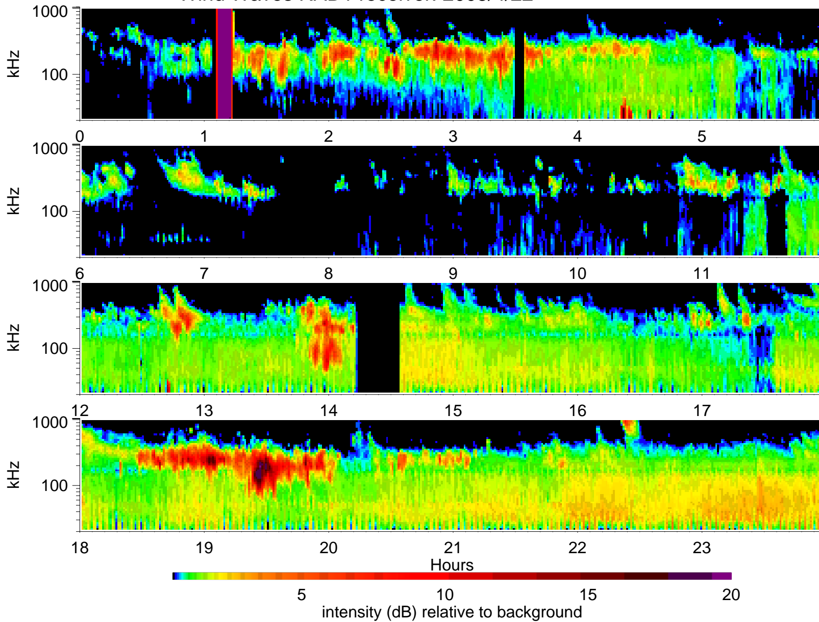
Wind Waves RAD1 receiver: 2005/4/22
