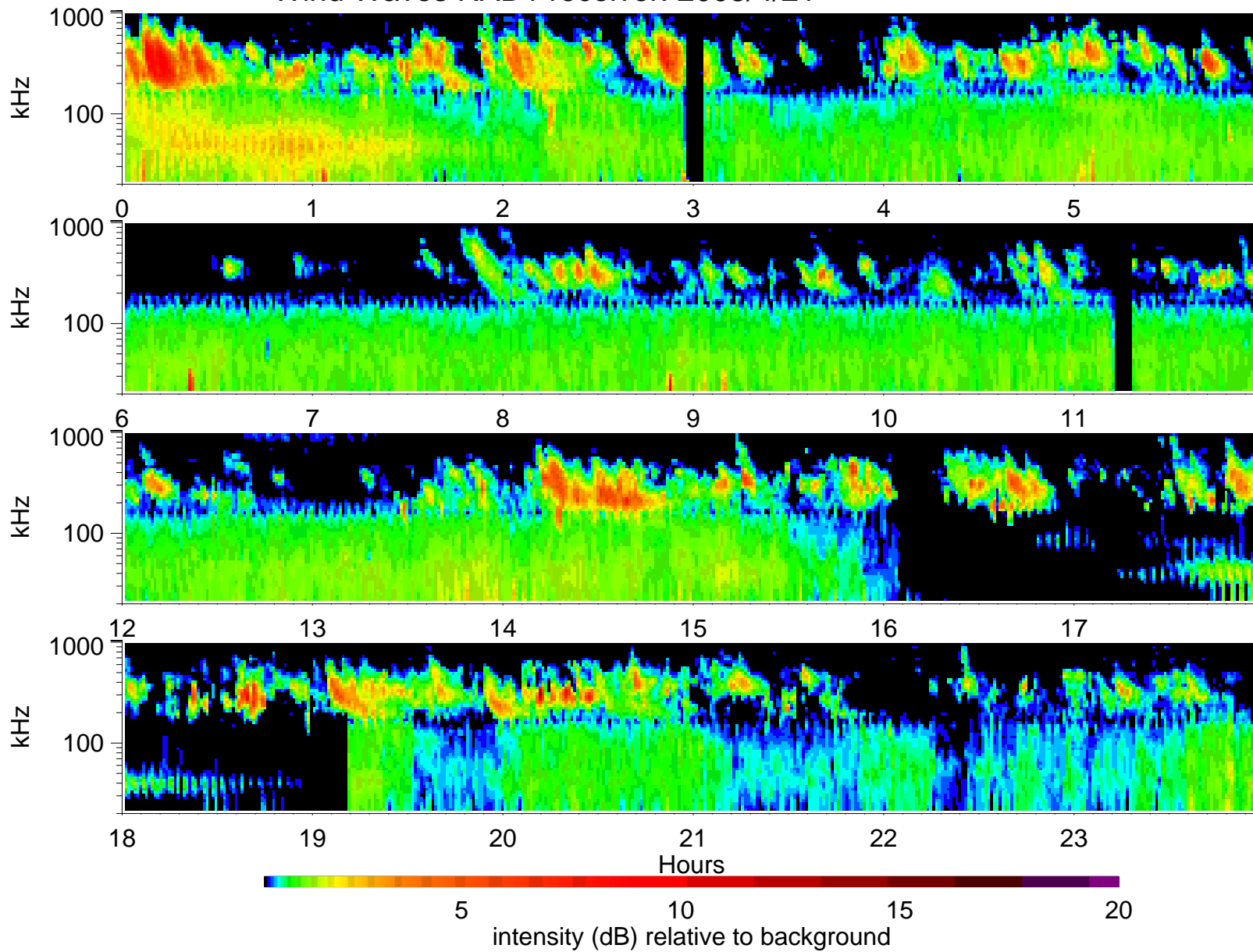
Wind Waves RAD1 receiver: 2005/4/21
