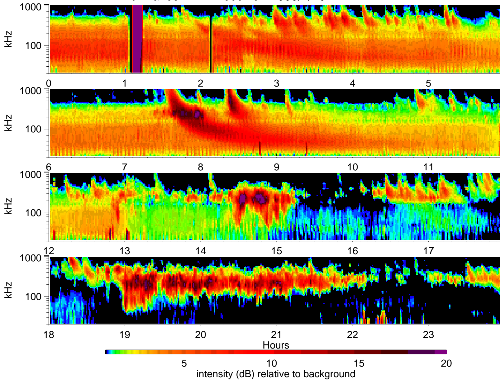
Wind Waves RAD1 receiver: 2005/4/20
