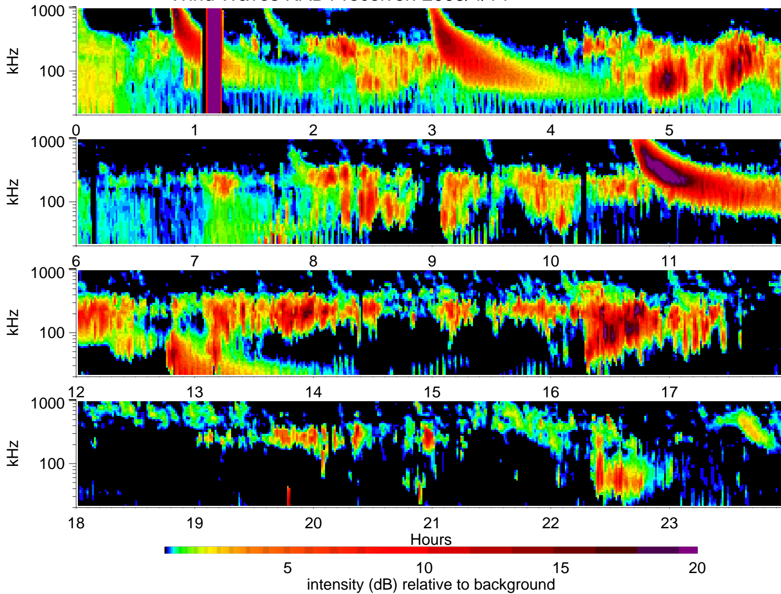
Wind Waves RAD1 receiver: 2005/4/14
