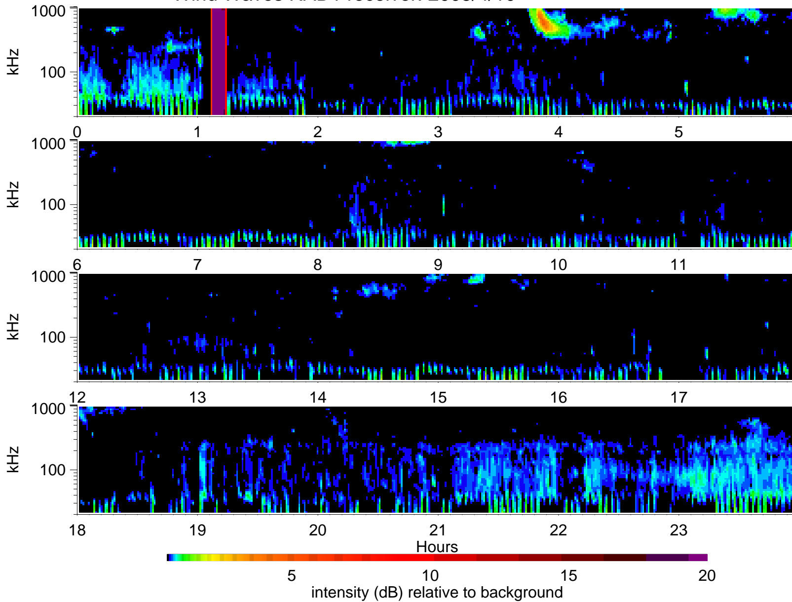
Wind Waves RAD1 receiver: 2005/4/10
