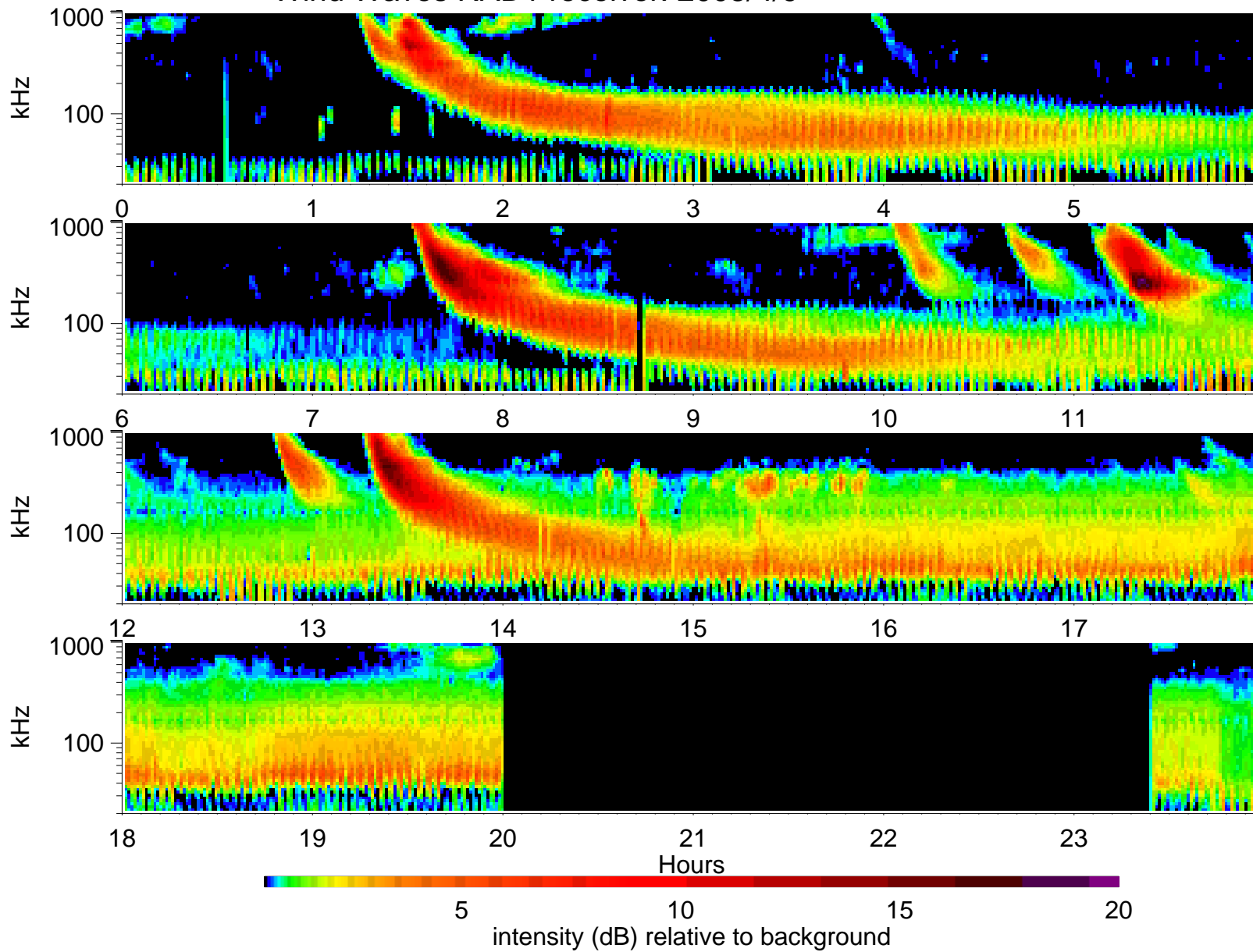
Wind Waves RAD1 receiver: 2005/4/9
