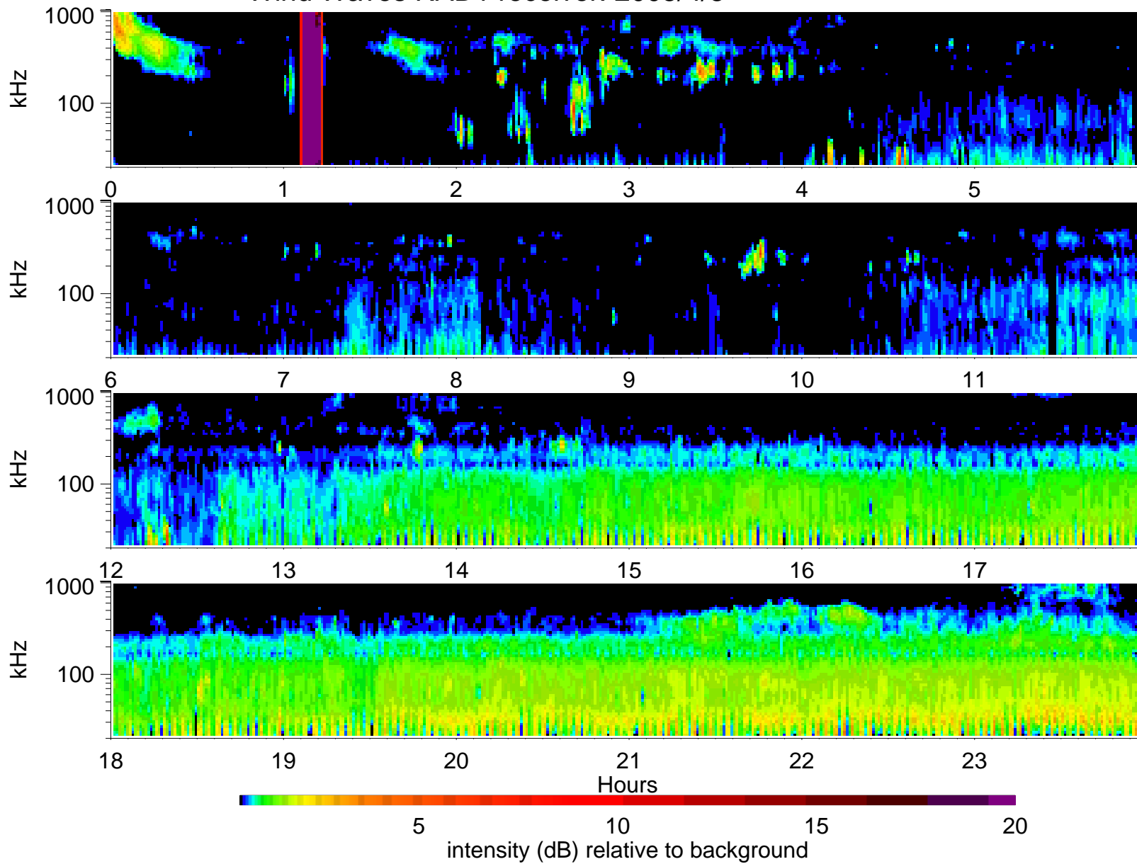
Wind Waves RAD1 receiver: 2005/4/8
