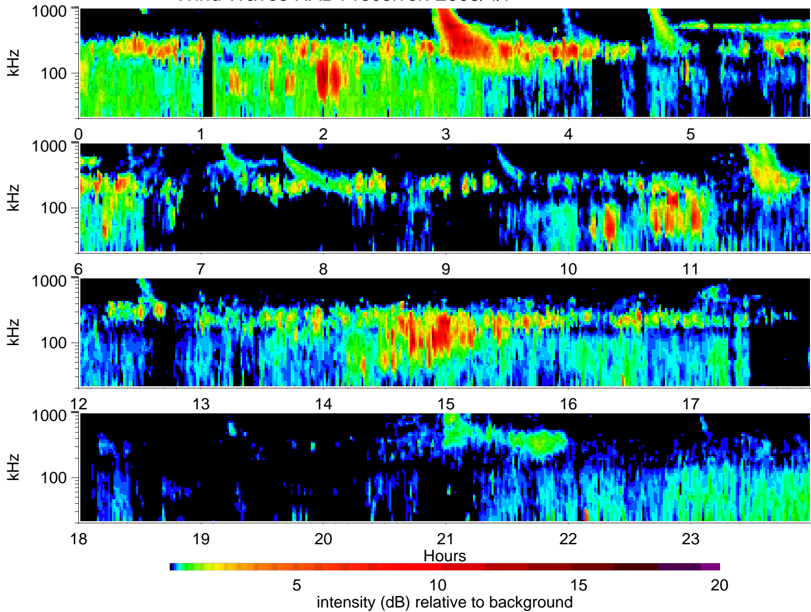
Wind Waves RAD1 receiver: 2005/4/7
