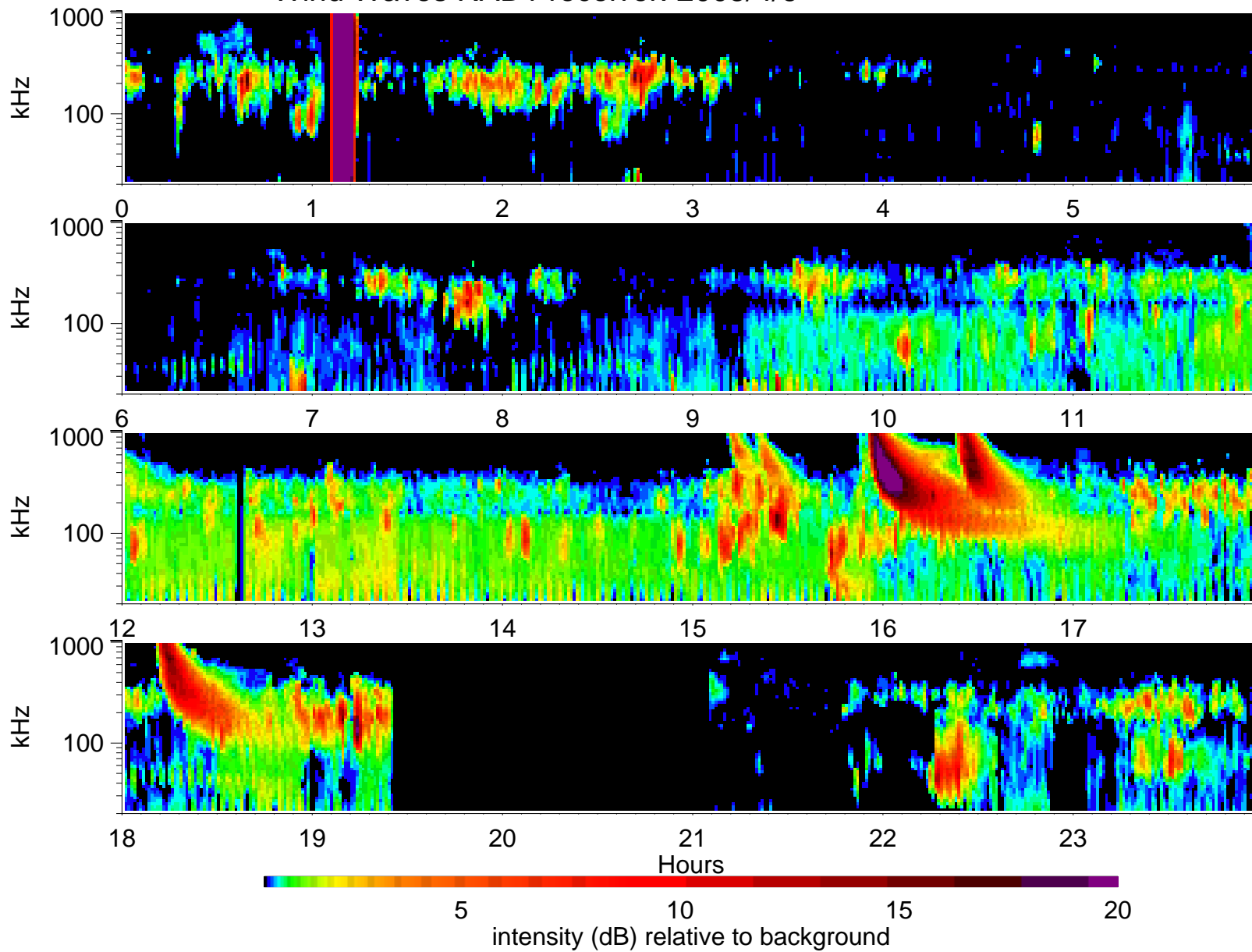
Wind Waves RAD1 receiver: 2005/4/6
