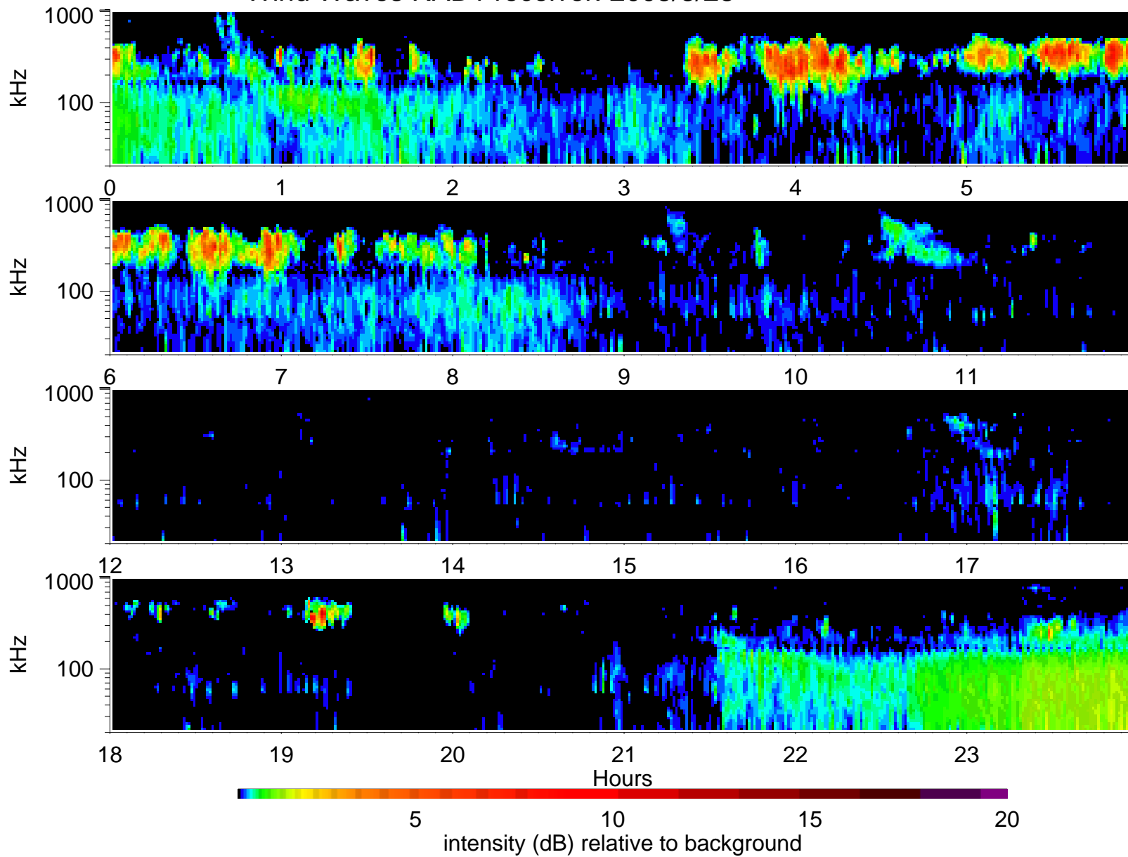
Wind Waves RAD1 receiver: 2005/3/28
