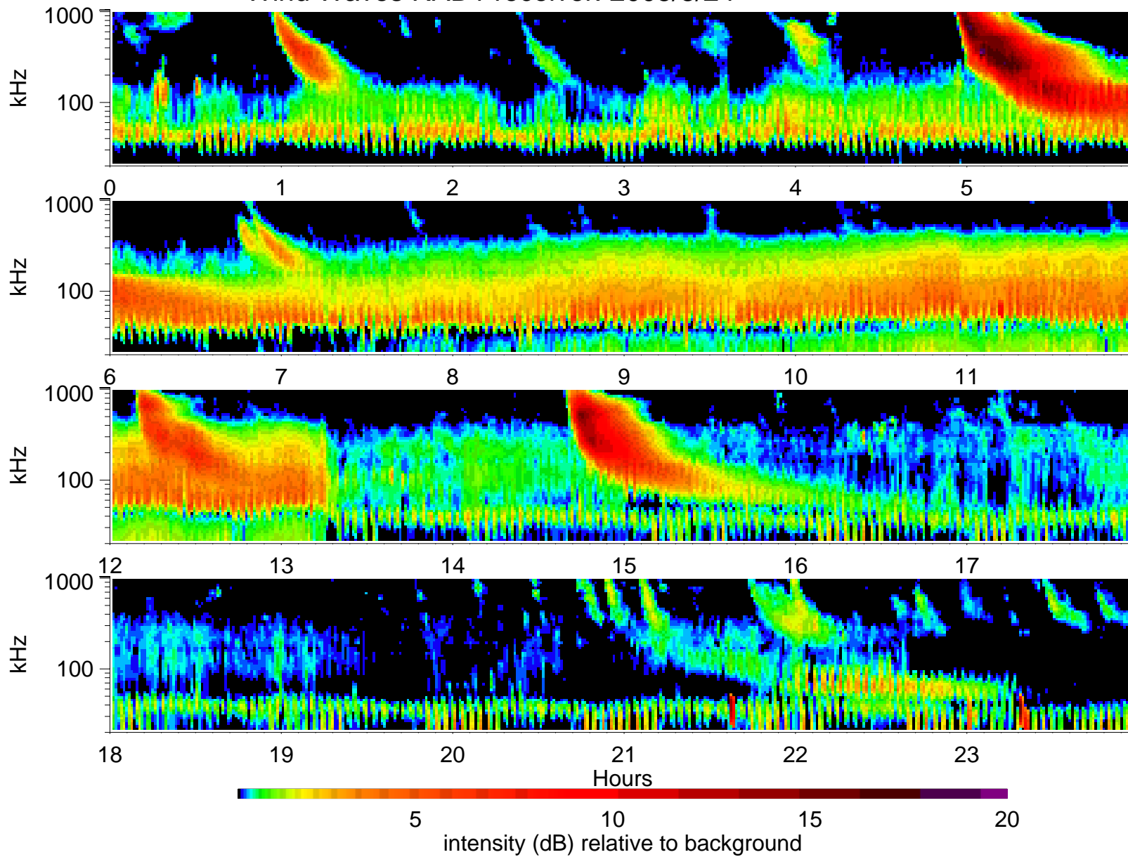
Wind Waves RAD1 receiver: 2005/3/24
