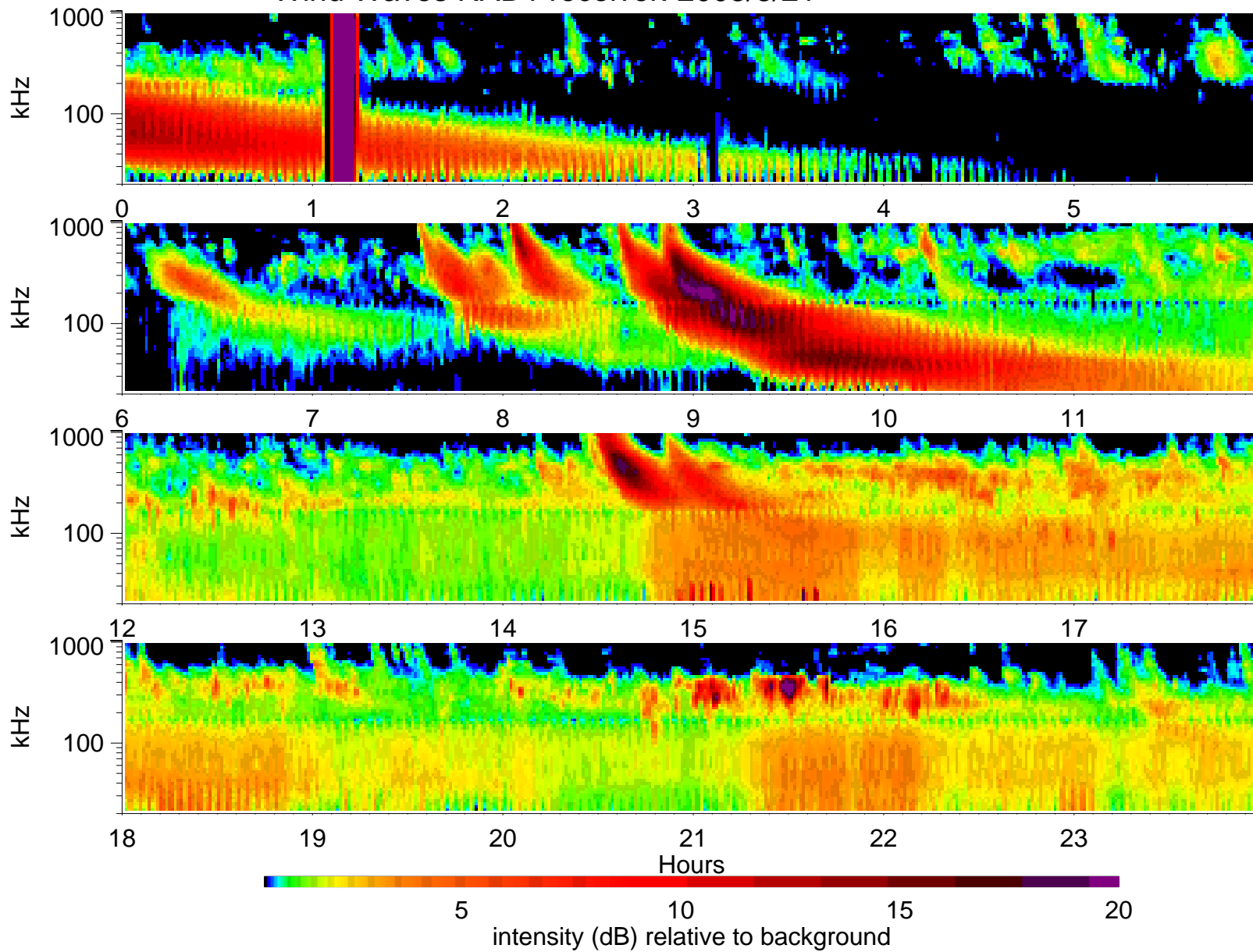
Wind Waves RAD1 receiver: 2005/3/21
