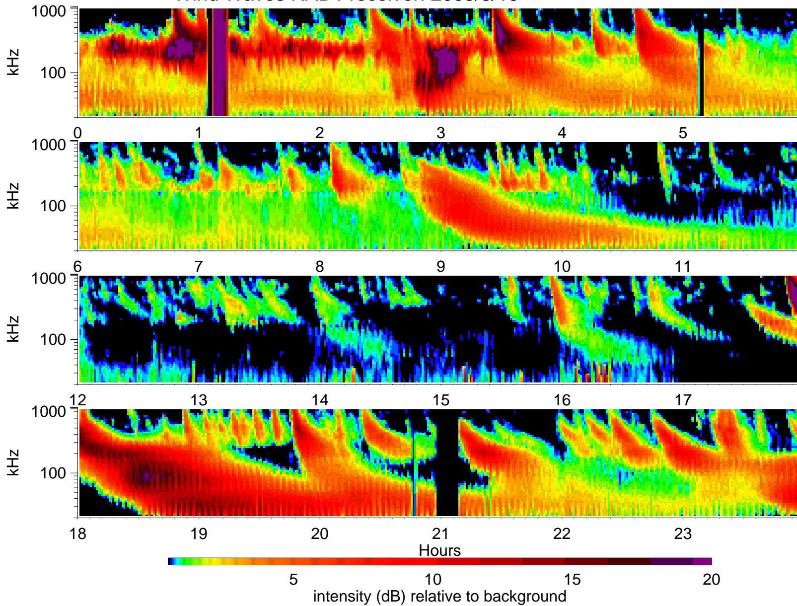
Wind Waves RAD1 receiver: 2005/3/19
