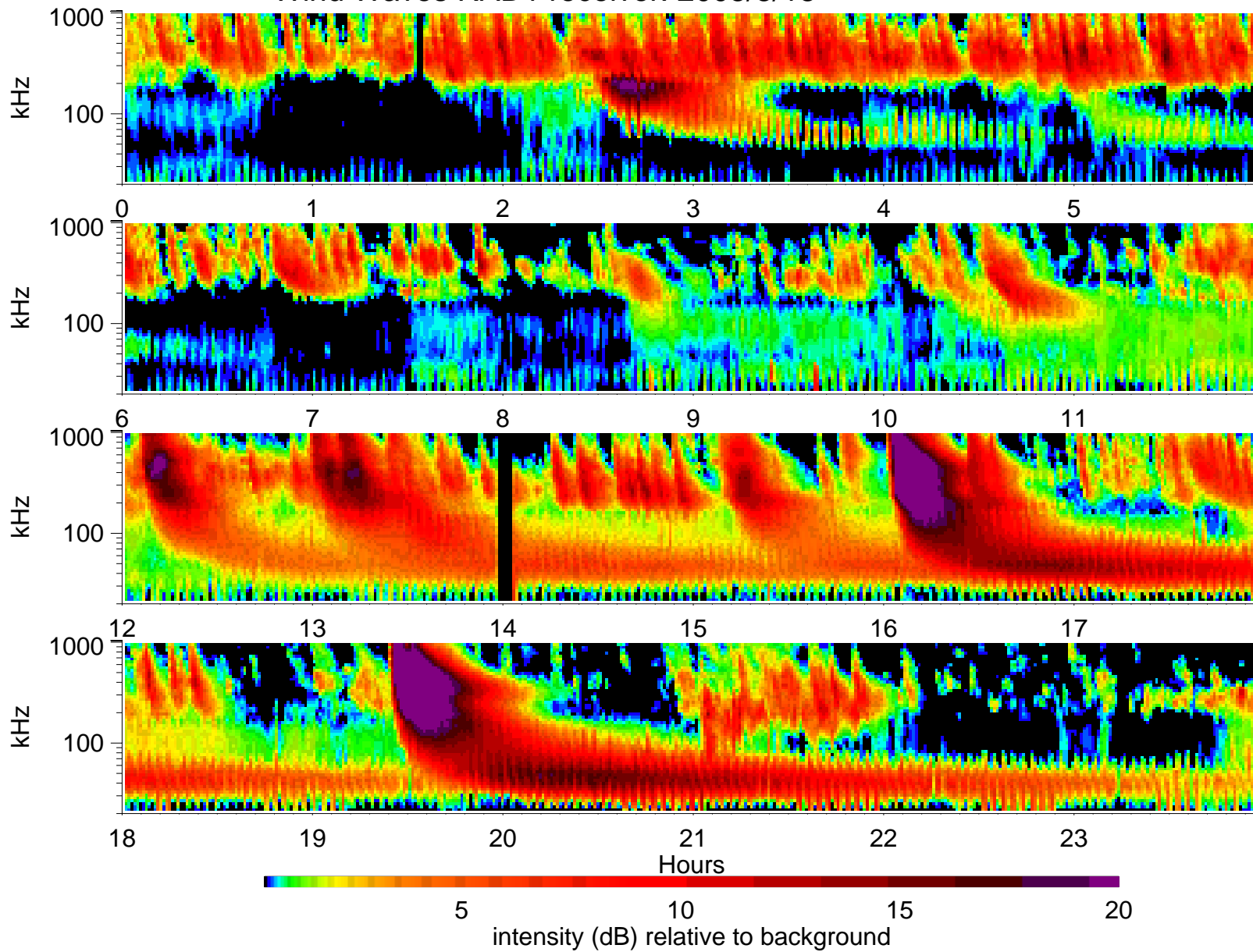
Wind Waves RAD1 receiver: 2005/3/18
