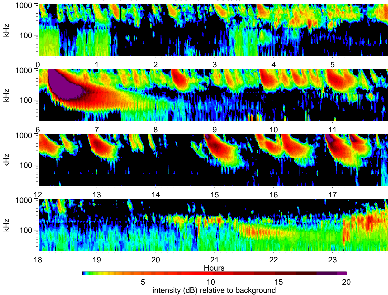
Wind Waves RAD1 receiver: 2005/3/12
