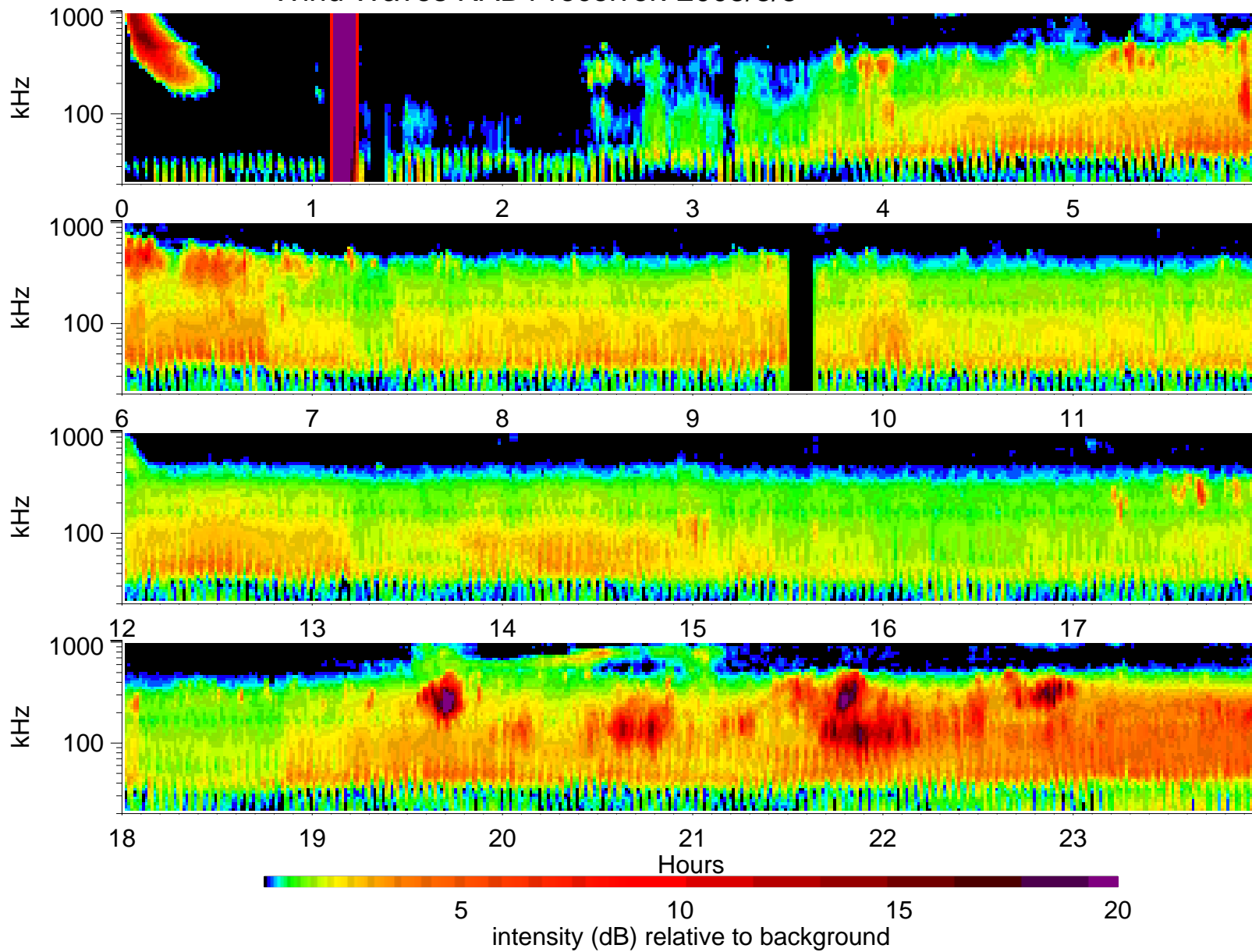
Wind Waves RAD1 receiver: 2005/3/5
