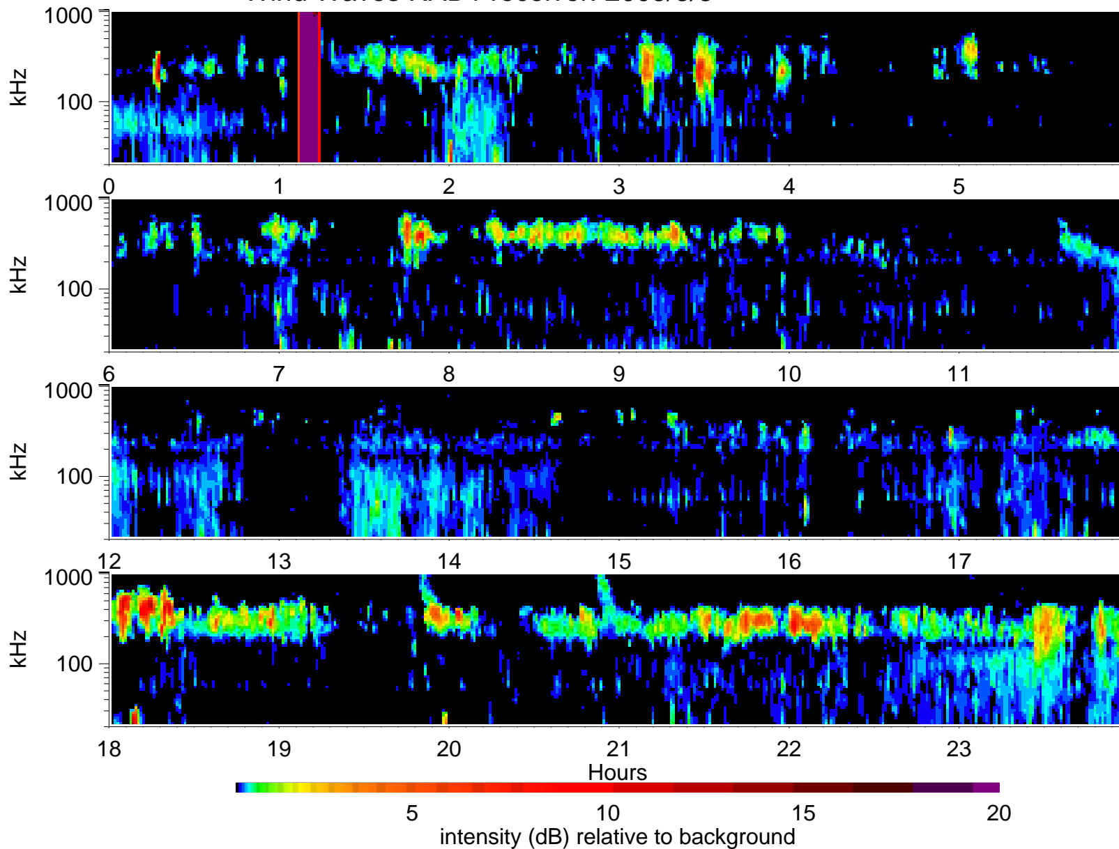
Wind Waves RAD1 receiver: 2005/3/3
