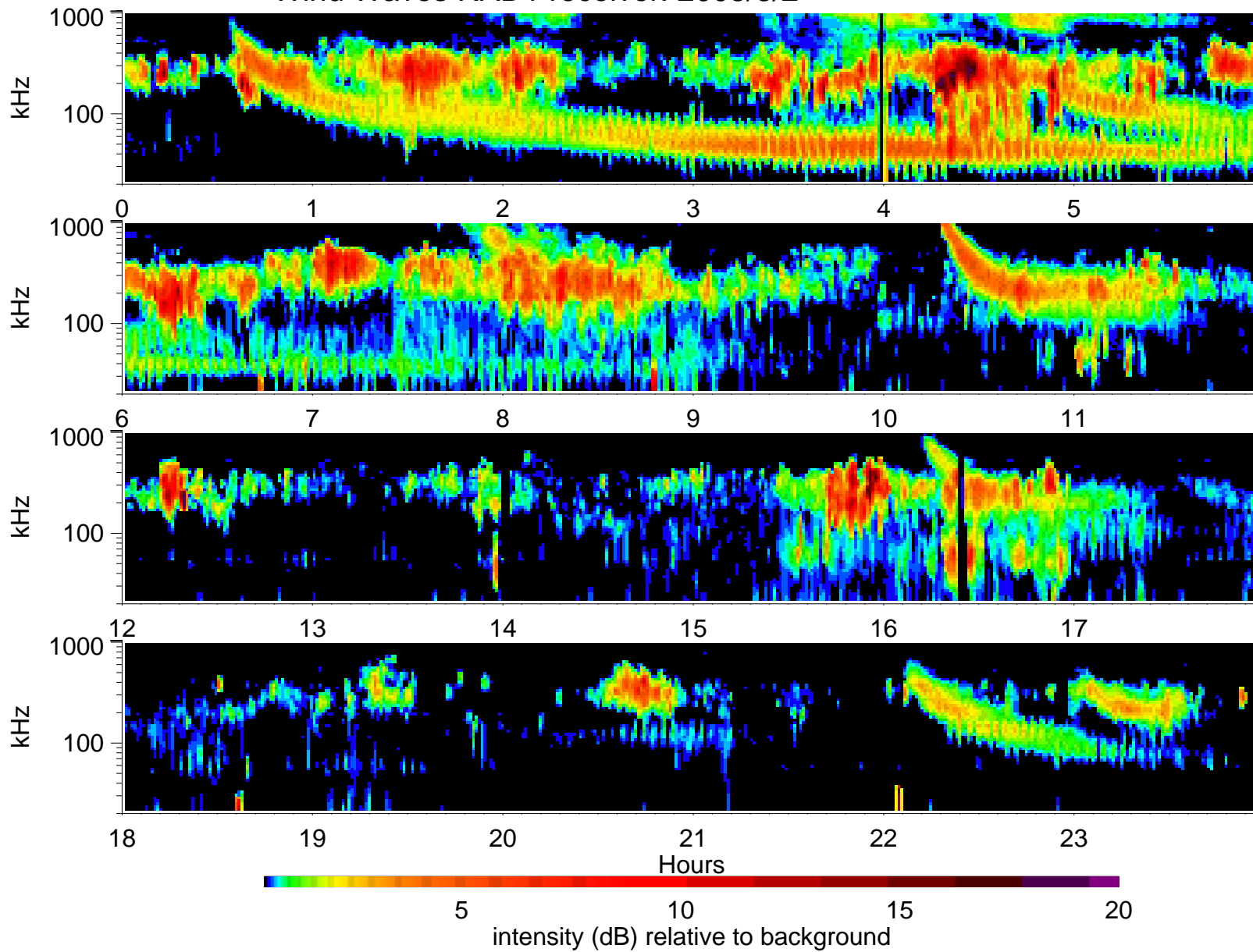
Wind Waves RAD1 receiver: 2005/3/2
