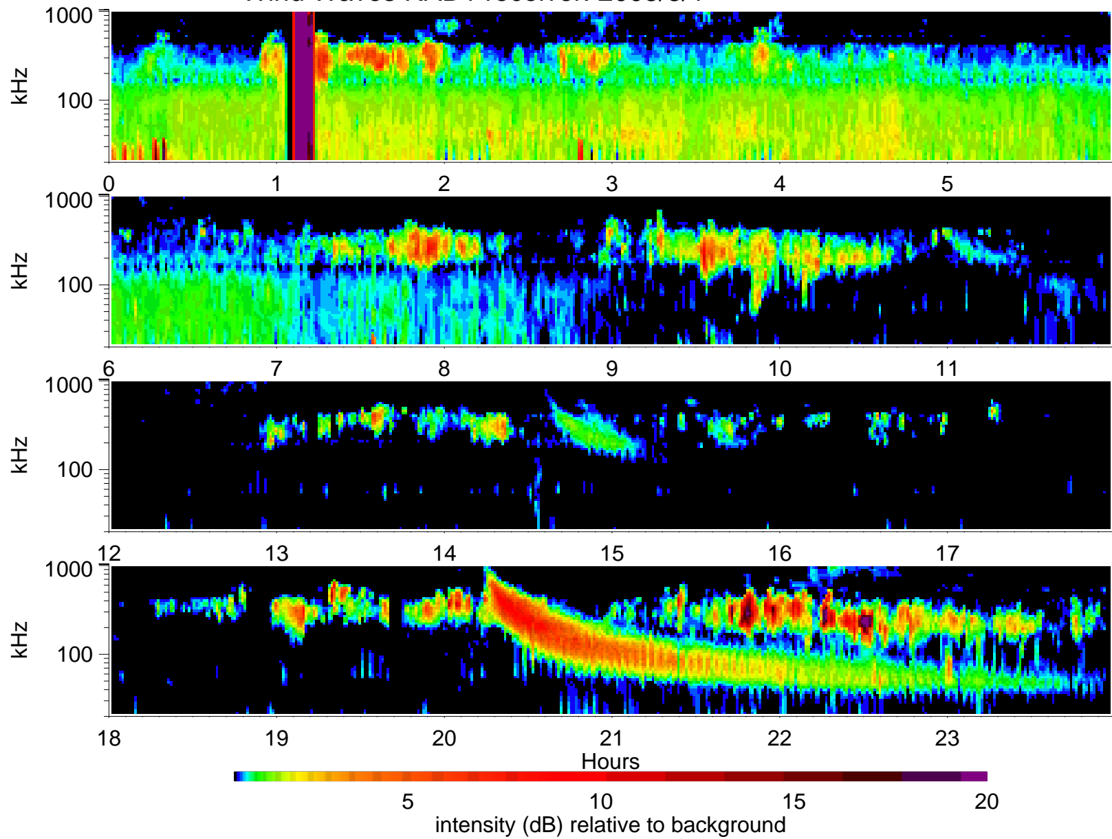
Wind Waves RAD1 receiver: 2005/3/1
