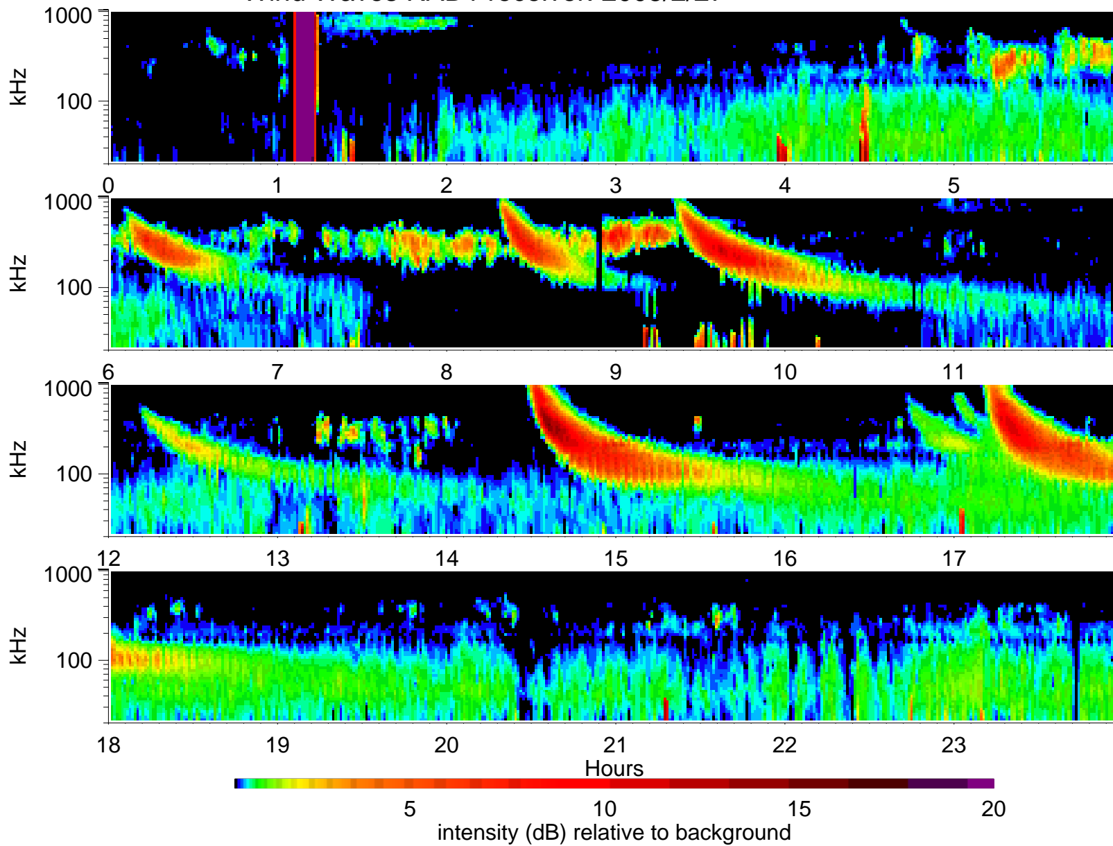
Wind Waves RAD1 receiver: 2005/2/27
