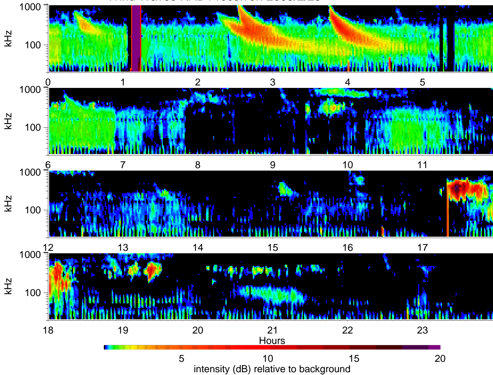
Wind Waves RAD1 receiver: 2005/2/25
