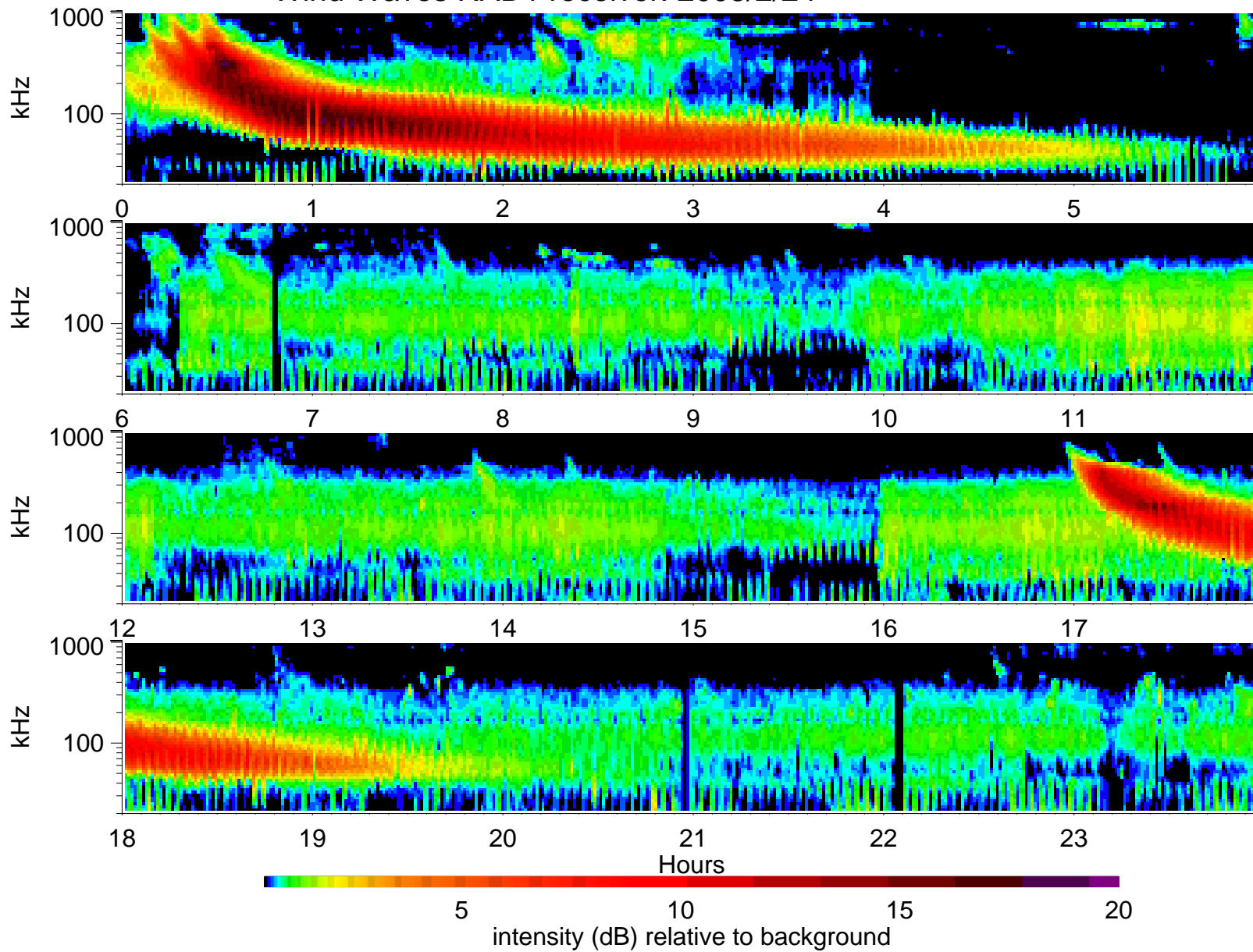
Wind Waves RAD1 receiver: 2005/2/24
